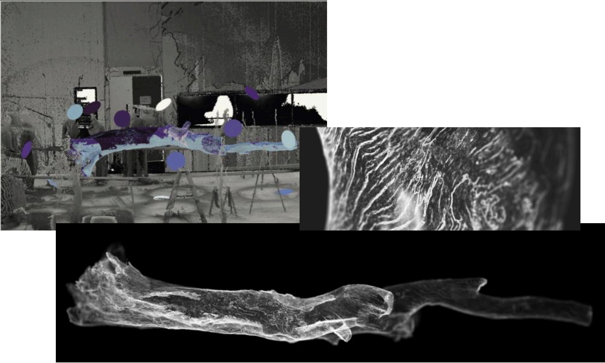
LiDAR scanning setup (top left) and 3D point cloud visualizations (black and white images).
