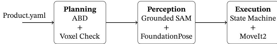
Figure 4.1: Overview of the three-stage pipeline.
