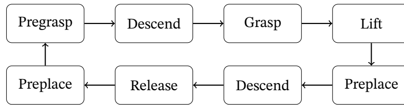
Figure 4.5: Overview of the execution state machine.
