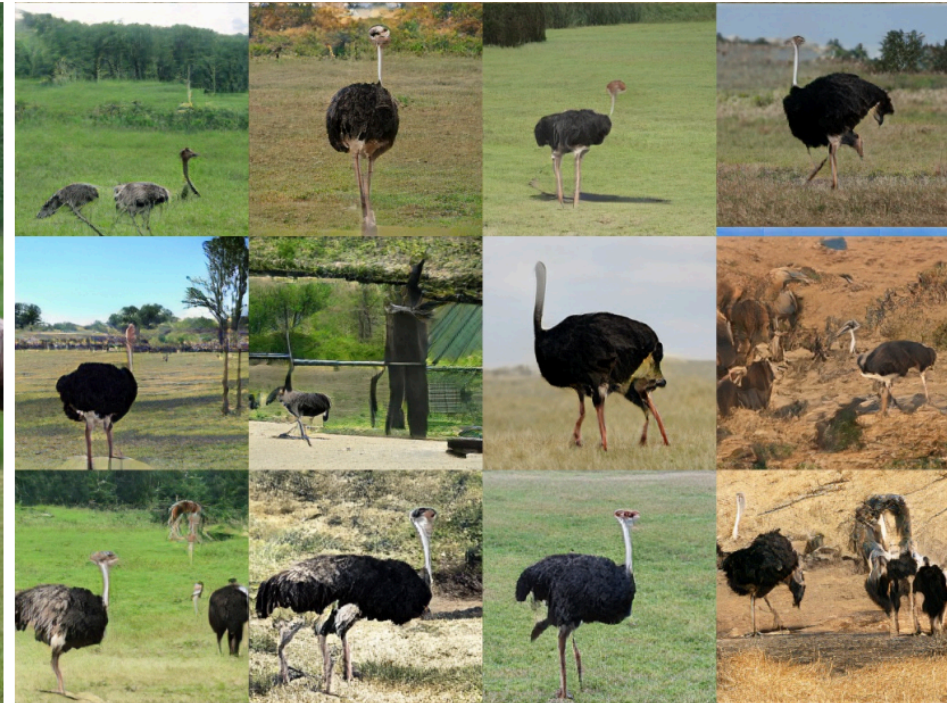
BigGAN deep
