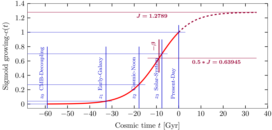
Figure 2: The C(t) curve of the compact sigmoid growing- c(t) model with determined parameters k = 0.1442 , \beta = 8.854 , t_w = -17.98 \text{ Gyr} , and J = 1.2789 . The corresponding cosmic times of the four benchmark epochs z_0, z_1, z_2, z_3 will be explained in Section 7.
