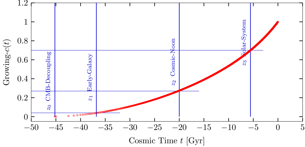
Figure 3: The C(t) curve of the ultra-fine growing- c(t) model, derived from Planck18 data. The corresponding cosmic times of the four benchmark epochs z_0, z_1, z_2, z_3 will be explained in the following section.
