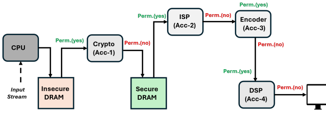
Fig. 2: A typical Multi-Accelerator SoC.
