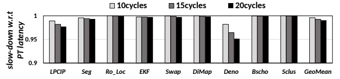
Fig. 19: Sensitivity to Permission Tracker latency.
