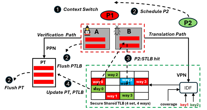
Fig. 12: ShareMMU-SP TLB set randomization.
