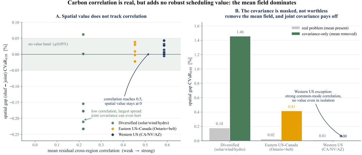
Figure 8: The Phase 1 finding. A: spatial gap vs. mean residual cross-region correlation; value does not track correlation anywhere on the spectrum. B: mean-leveling test; in the covariance-only world (constant scheduling mean) the joint covariance pays off by up to +1.46%, proving the spatial signal is real but masked by the mean carbon field, not absent.
