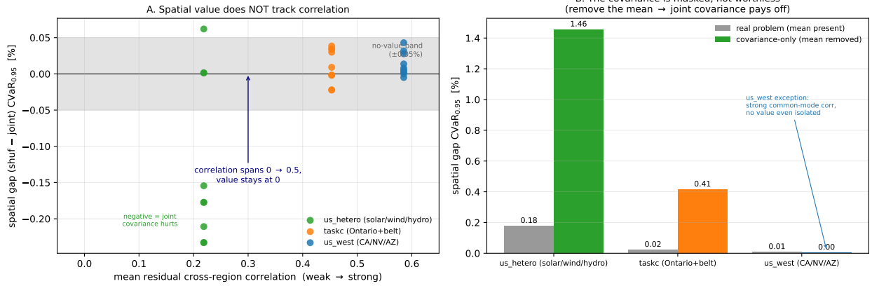
Figure 2: The Phase 1 finding. A: spatial gap vs. mean residual cross-region correlation (value does not track correlation anywhere on the spectrum). B: mean-ablation) in the covariance-only world (constant scheduling mean) the joint covariance pays off by up to +1.46%, proving the spatial signal is real but masked by the mean carbon field, not absent.
