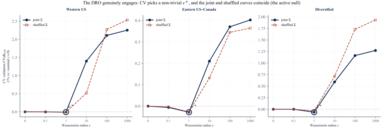
Figure 6: The DRO genuinely engages. Blocked 5-fold cross-validation \text{CVaR}_{0.95} (relative to the nominal \varepsilon = 0 problem) against the Wasserstein radius \varepsilon , for the joint (solid) and shuffled (dashed) covariances. Cross-validation selects an interior \varepsilon^* (circled), not \varepsilon = 0 , so the robustification is on; the two curves coincide, so the spatial covariance changes nothing. Large \varepsilon is over-conservative.
