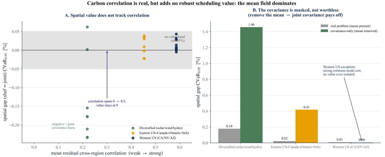
Figure 7: The Phase 1 finding. A: spatial gap vs. mean residual cross-region correlation; value does not track correlation anywhere on the spectrum. B: mean-ablation; in the covariance-only world (constant scheduling mean) the joint covariance pays off by up to +1.46%, proving the spatial signal is real but masked by the mean carbon field, not absent.
