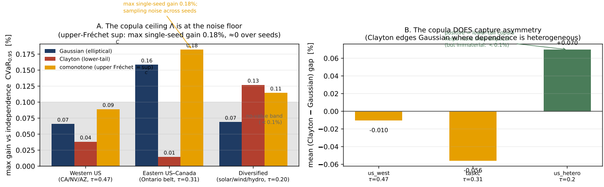
Figure 11: Phase 2 result (single locked scenario seed). A: maximum positive gain versus independence for the Gaussian, Clayton, and comonotone (upper-Fréchet sup C ) arms. The largest single-seed comonotone gain is 0.18% (Eastern US-Canada); re-evaluated over scenario seeds it is sampling noise centred on zero (Figure 13). B: the mean Clayton-Gaussian increment by grid; positive where dependence is heterogeneous (Diversified, +0.07%), confirming the copula does capture the asymmetry, but an order of magnitude too small to matter, as Proposition 1 predicts.
