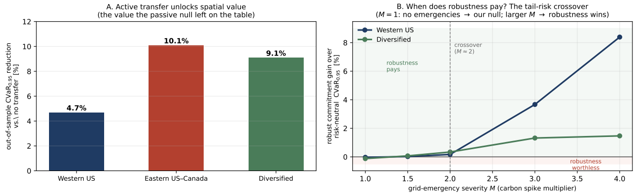
Figure 13: Preliminary Phase 3. A: active transfer reduces out-of-sample \text{CVaR}_{0.95} by 4.7–10.1%. B: the tail-risk crossover, the robust (CVaR-hedged) commitment’s advantage over the risk-neutral one as grid-emergency severity M grows; near M \approx 2 it turns positive. Proof-of-concept; full treatment is future work.
