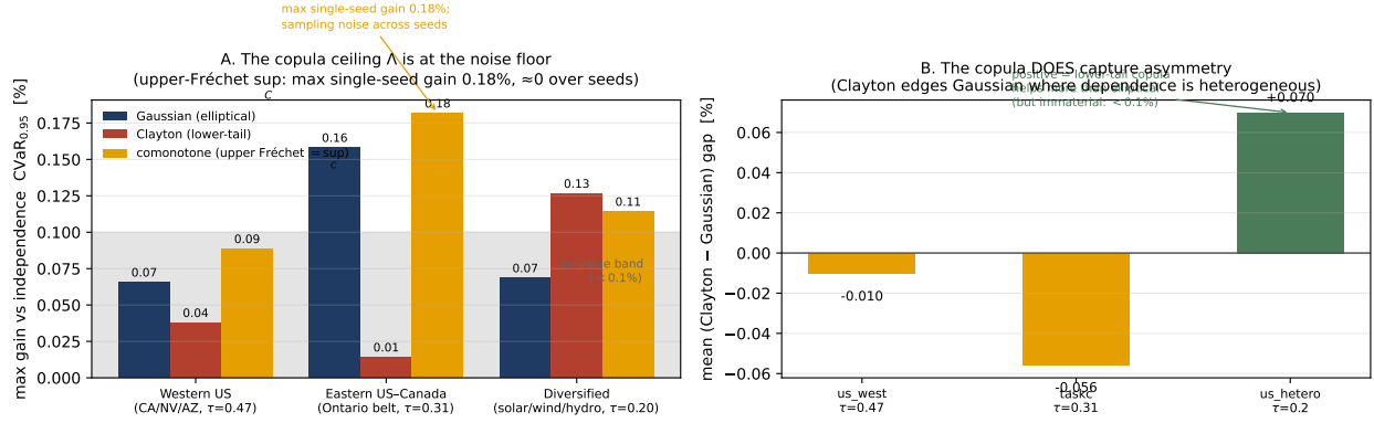
Figure 10: Phase 2 result (single locked scenario seed). A: maximum positive gain versus independence for the Gaussian, Clayton, and comonotone (upper-Fréchet sup C ) arms. The largest single-seed comonotone gain is 0.18% (Eastern US-Canada); re-evaluated over scenario seeds it is sampling noise centred on zero (Figure 12). B: the mean Clayton-Gaussian increment by grid; positive where dependence is heterogeneous (Diversified, +0.07%), confirming the copula does capture the asymmetry, but an order of magnitude too small to matter, as Proposition 1 predicts.
