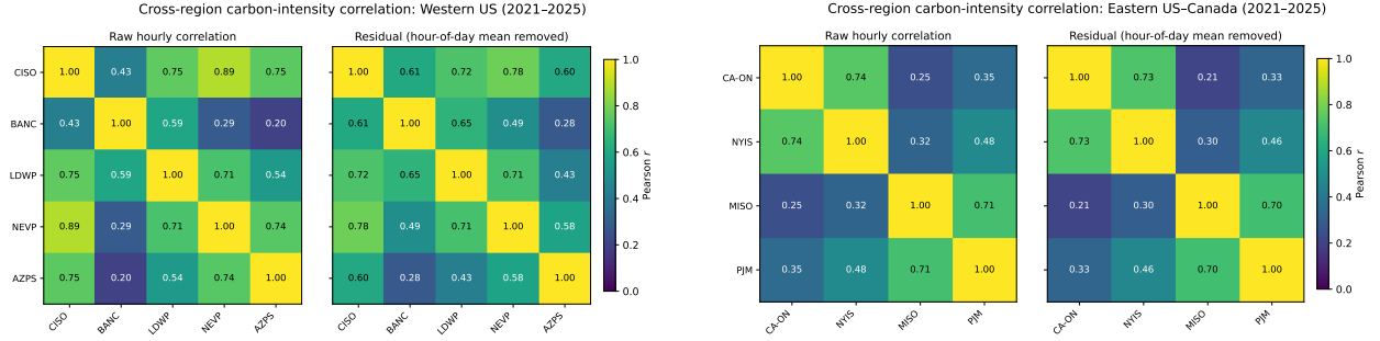
Figure 2: Residual (hour-of-day-removed) cross-region correlation of hourly carbon intensity, 2021–2025. Left: US West (CISO, BANC, LDWP, NEVP, AZPS). Right: Ontario–Eastern belt (CA-ON, NYIS, MISO, PJM). Spatial correlation is strong and genuine in both, the assumption motivating spatial DRO is empirically valid.
