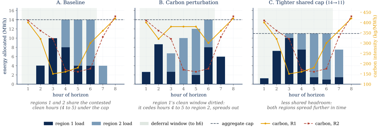
Figure 1: Full-model validation on a two-region instance. The complete feasible set (capacity, work conservation, ramp, deferral deadline) plus a shared aggregate hourly cap is solved jointly; stacked bars show how the two regions share each hour, the dashed line is the aggregate cap, the curves are each region's carbon field, the green band the deadline window. A: baseline, the regions split the contested clean hours (4–5) under the cap. B: after dirtying region 1's clean window, it cedes those hours to region 2 and spreads out. C: after tightening the shared cap, both regions spread further in time. Each response is the one an analyst anticipates, confirming the model encodes the intended cross-region behaviour.
