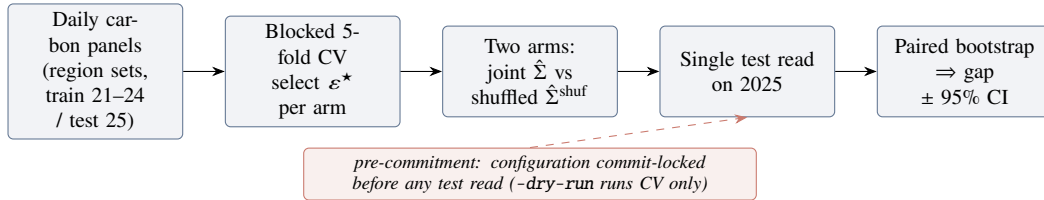
Figure 2: The pre-committed falsification pipeline. Cross-validation and schedule fitting touch only the training years; the 2025 test set is read once, after the configuration is commit-locked, and the spatial gap is read off a paired day-bootstrap.
