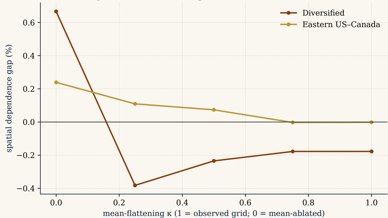
Dependence value emerges as mean differences flatten
