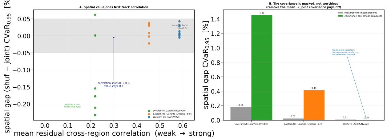
Figure 8: The Phase 1 finding. A: spatial gap vs. mean residual cross-region correlation; value does not track correlation anywhere on the spectrum. B: mean-leveling test; in the covariance-only world (constant scheduling mean) the joint covariance pays off by up to +1.46%, proving the spatial signal is real but masked by the mean carbon field, not absent.
