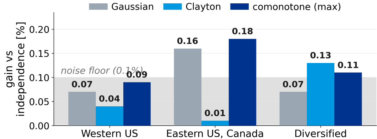
Figure 21: Copula result (single locked scenario seed). A: maximum positive gain versus independence for the Gaussian, Clayton, and comonotone (upper-Fréchet \sup_C ) arms. The largest single-seed comonotone gain is 0.18% (Eastern US–Canada); re-evaluated over scenario seeds it is sampling noise centred on zero (Figure 19). B: the mean Clayton–Gaussian increment by grid; positive where dependence is heterogeneous (Diversified, +0.07%), confirming the copula does capture the asymmetry, but an order of magnitude too small to matter, as Proposition 1 predicts.
