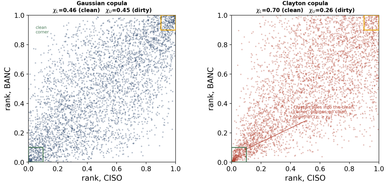
Figure 20: The dependence object a covariance ball cannot represent. Samples from the Gaussian copula (left, symmetric: \chi_L \approx \chi_U ) and the fitted Clayton copula (right) for a representative US-West pair. Clayton concentrates in the lower-left “clean” corner ( \chi_L > \chi_U ), reproducing the Phase 1 radial asymmetry that elliptical models force to zero.
