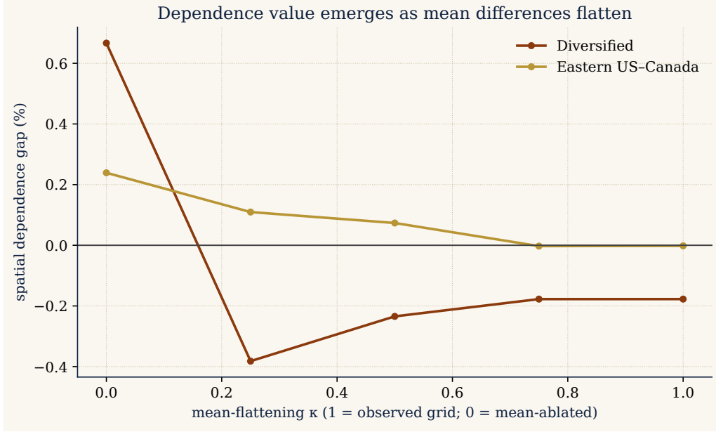
Figure 17: Interior validation of the Part 5 condition. Realised spatial gap (% of \text{CVaR}_{0.95} ) from re-solving the DRO at intermediate mean-flattenings \kappa . On the correlated Eastern grid the gap rises monotonically as the mean weakens ( \kappa \rightarrow 0 ), tracking \Delta ; on the engineered Diversified grid it is non-monotone, the joint covariance fitting noise before the true signal emerges, so \Delta orders the regimes only coarsely.
