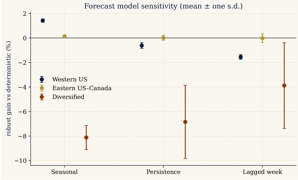
Figure 16: Part 4 forecast robustness. Online robust-vs-deterministic gap (% of \text{CVaR}_{0.95} , three seeds) under three day-ahead forecasts. On the correlated grids the sign flips with the forecast (immaterial); on Diversified the robust controller loses under every forecast.
