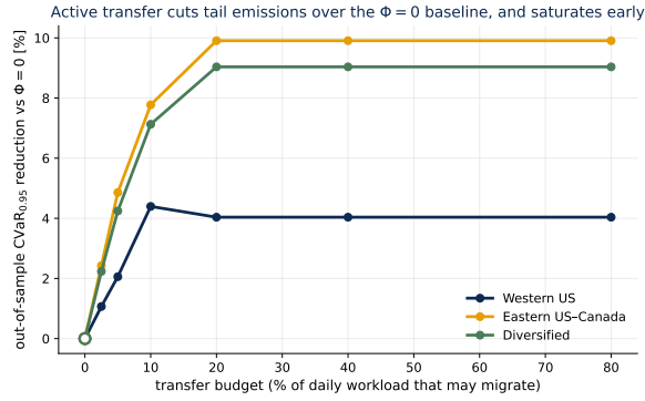
Figure 4: The transfer lever. Out-of-sample CVaR 0.95 saving against the inter-region transfer budget \Phi , relative to the carbon-aware no-transfer baseline ( \Phi = 0 ). Active migration captures this spatial lever; the curve saturates as the feasible mean-based gain is exhausted. The robust layer is analyzed in Section 4.9.
