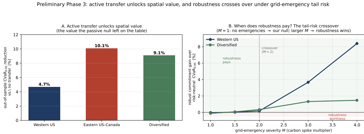
Figure 13: Preliminary Phase 3. A: active transfer reduces out-of-sample \text{CVaR}_{0.95} by 4.7–10.1%. B: the tail-risk crossover — the robust (CVaR-hedged) commitment’s advantage over the risk-neutral one as grid-emergency severity M grows; near M \approx 2 it turns positive. Proof-of-concept; full treatment is future work.
