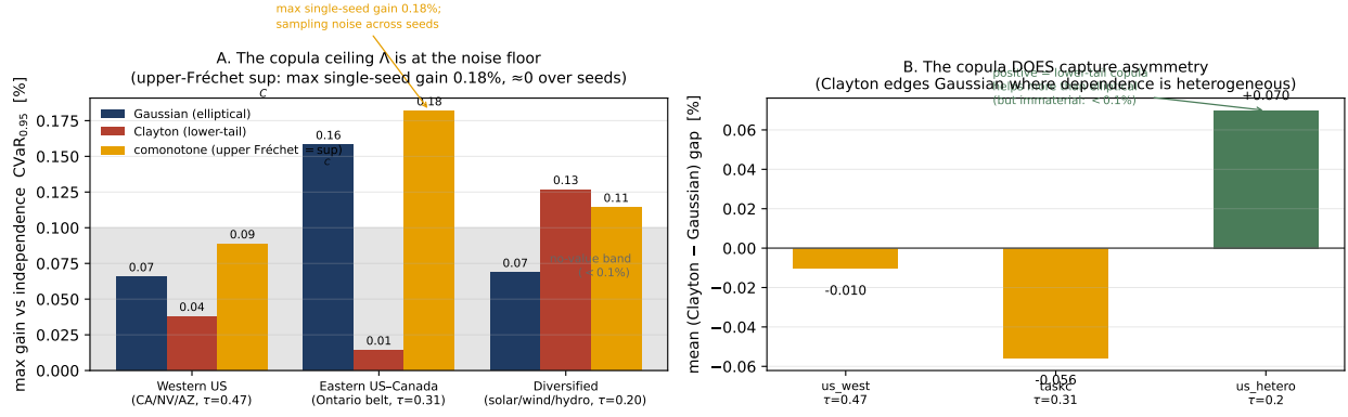
Figure 10: Phase 2 result (single locked scenario seed). A: maximum positive gain versus independence for the Gaussian, Clayton, and comonotone (upper-Fréchet sup C ) arms. The largest single-seed comonotone gain is 0.18% (Eastern US-Canada); re-evaluated over scenario seeds it is sampling noise centred on zero (Figure 12). B: the mean Clayton-Gaussian increment by grid; positive where dependence is heterogeneous (Diversified, +0.07%), confirming the copula does capture the asymmetry, but an order of magnitude too small to matter, as Proposition 1 predicts.
