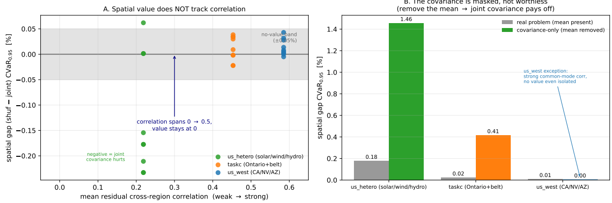
Figure 2: The Phase 1 finding. A : spatial gap vs. mean residual cross-region correlation — value does not track correlation anywhere on the spectrum. B : mean-ablation — in the covariance-only world (constant scheduling mean) the joint covariance pays off by up to +1.46%, proving the spatial signal is real but masked by the mean carbon field, not absent.
