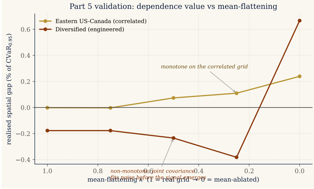
Figure 15: Interior validation of the Part 5 condition. Realised spatial gap (% of \text{CVaR}_{0.95} ) from re-solving the DRO at intermediate mean-flattenings \kappa . On the correlated Eastern grid the gap rises monotonically as the mean weakens ( \kappa \rightarrow 0 ), tracking \Delta ; on the engineered Diversified grid it is non-monotone, the joint covariance fitting noise before the true signal emerges, so \Delta orders the regimes only coarsely.
