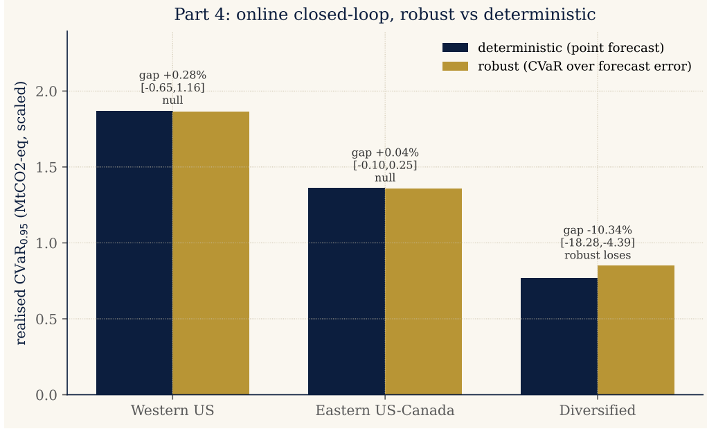
Figure 14: Part 4. Realised closed-loop CVaR 0.95 , deterministic vs robust controller, per grid; annotations give the robust gap and its 95% CI. Robustness is null on the correlated grids and counterproductive on the structureless one.
