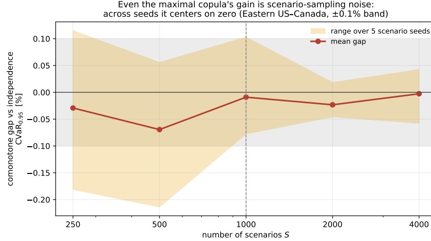
Figure 19: The comonotone gap is scenario-sampling noise. Mean (line) and range over five seeds (band) of the comonotone-vs-independence \text{CVaR}_{0.95} gap on Eastern US–Canada, against the scenario count S . The band straddles zero and narrows with S ; the \pm 0.1\% no-value band is shaded.
