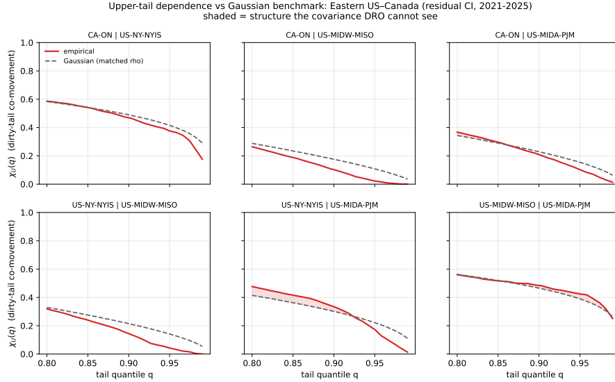
Figure 9: Upper-tail dependence \chi_U(q) for the Ontario–Eastern belt region pairs (solid) against the Gaussian-copula benchmark at the matched correlation (dashed). The empirical curves sit at or below the benchmark as q \rightarrow 1 : in the dirtiest hours the regions decouple, so there is no exploitable upper-tail co-movement for a richer ambiguity set to capture. The complementary radial asymmetry ( \chi_L > \chi_U ) is quantified in Table 6.
