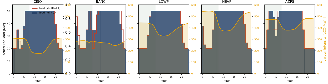
Figure 6: The spatial null, seen directly (Western US, regime R3, \alpha = 0.5 , \varepsilon^* = 1 ). Bars are the optimal load under the joint covariance; the red step is the load under the shuffled (block-diagonal) covariance. The two coincide. The gold curve is each region’s mean carbon intensity; the green band marks the deadline window [0, 7] .
