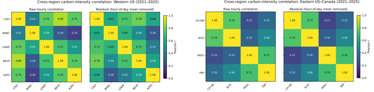
Figure 2: Residual (hour-of-day-removed) cross-region correlation of hourly carbon intensity, 2021–2025. Left: US West (CISO, BANC, LDWP, NEVP, AZPS). Right: Ontario–Eastern belt (CA-ON, NYISO, MISO, PJM). Spatial correlation is strong and genuine in both, the assumption motivating spatial DRO is empirically valid.
