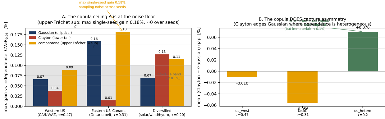
Figure 10: Phase 2 result (single locked scenario seed). A: maximum positive gain versus independence for the Gaussian, Clayton, and comonotone (upper-Fréchet \sup_C ) arms. The largest single-seed comonotone gain is 0.18% (Eastern US-Canada); re-evaluated over scenario seeds it is sampling noise centred on zero (Figure 12). B: the mean Clayton-Gaussian increment by grid; positive where dependence is heterogeneous (Diversified, +0.07%), confirming the copula does capture the asymmetry, but an order of magnitude too small to matter, as Proposition 1 predicts.
