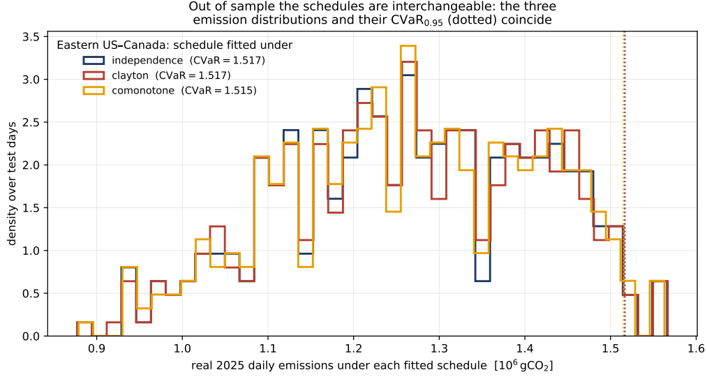
Figure 11: Out of sample the copula schedulers are interchangeable (Eastern US–Canada). Distribution of real 2025 daily emissions under the schedule fitted to independence, Clayton, and comonotone scenarios; the dotted lines mark each \text{CVaR}_{0.95} . All three coincide.
