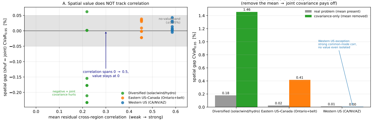
Figure 5: The Phase 1 finding. A: spatial gap vs. mean residual cross-region correlation; value does not track correlation anywhere on the spectrum. B: mean-ablation; in the covariance-only world (constant scheduling mean) the joint covariance pays off by up to +1.46%, proving the spatial signal is real but masked by the mean carbon field, not absent.
