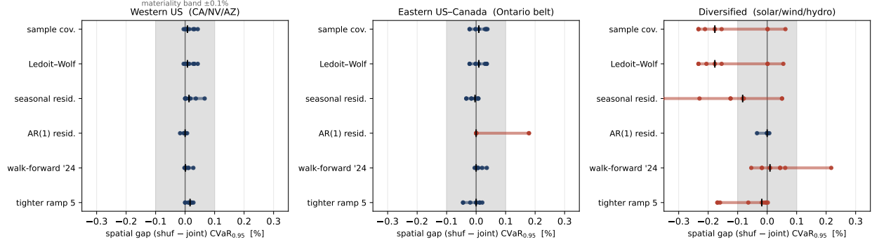
Figure 7: Robustness of the null. For each grid and each robustness arm (sample covariance, Ledoit–Wolf, seasonal and AR(1) residuals, walk-forward to 2024, and a 3\times tighter ramp), dots are the spatial gap for the nine (regime, \alpha ) cells and the tick marks the median. The shaded band is the \pm 0.1\% materiality threshold. No arm produces a sign-stable, material gap; the few Diversified excursions are negative (the joint covariance mildly hurts).
