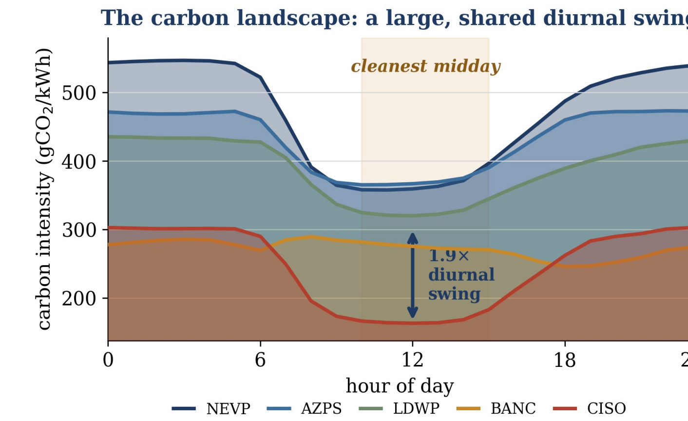
The dominant mean carbon field : the schedule follows this terrain; the spatial covariance is a thin ripple on top (≤1.46%).
