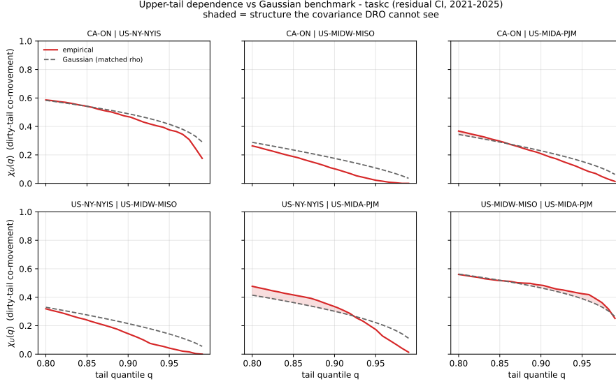
Figure 7: Upper-tail dependence \chi_U(q) for the Ontario–Eastern belt region pairs (solid) against the Gaussian-copula benchmark at the matched correlation (dashed). The empirical curves sit at or below the benchmark as q \rightarrow 1 : in the dirtiest hours the regions decouple, so there is no exploitable upper-tail co-movement for a richer ambiguity set to capture. The complementary radial asymmetry ( \chi_L > \chi_U ) is quantified in Table 4.
