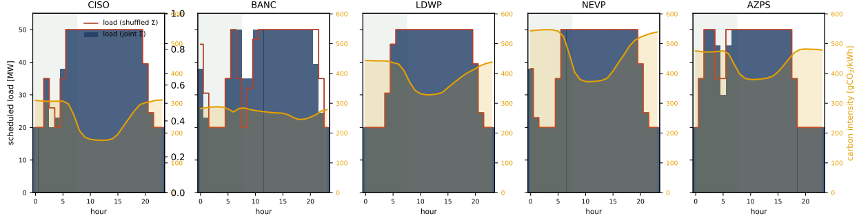
Figure 5: The spatial null, seen directly (us_west, regime R3, \alpha = 0.5 , \varepsilon^* = 1 ). Bars are the optimal load under the joint covariance; the red step is the load under the shuffled (block-diagonal) covariance. The two coincide. The gold curve is each region’s mean carbon intensity; the green band marks the deadline window [0, 7] .
