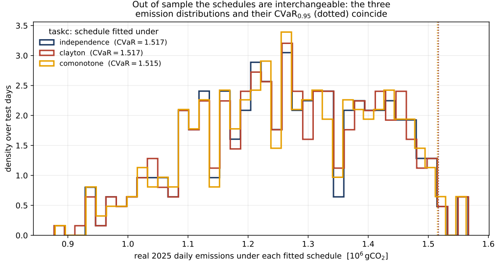
Figure 10: Out of sample the copula schedulers are interchangeable (taskc). Distribution of real 2025 daily emissions under the schedule fitted to independence, Clayton, and comonotone scenarios; the dotted lines mark each \text{CVaR}_{0.95} . All three coincide.
