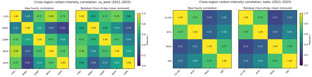
Figure 1: Residual (hour-of-day-removed) cross-region correlation of hourly carbon intensity, 2021–2025. Left: US West (CISO, BANC, LDWP, NEVP, AZPS). Right: Ontario–Eastern belt (CA-ON, NYIS, MISO, PJM). Spatial correlation is strong and genuine in both, the assumption motivating spatial DRO is empirically valid.
