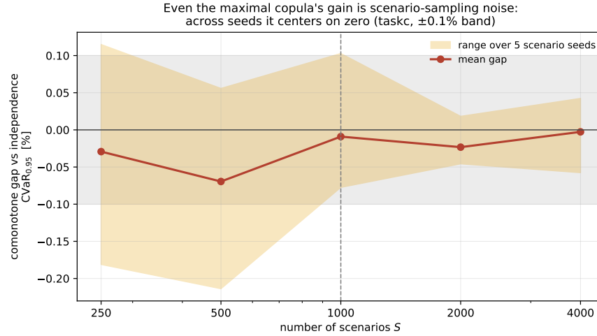
Figure 11: The comonotone gap is scenario-sampling noise. Mean (line) and range over five seeds (band) of the comonotone-vs-independence \text{CVaR}_{0.95} gap on taskc , against the scenario count S . The band straddles zero and narrows with S ; the \pm 0.1\% materiality band is shaded.
