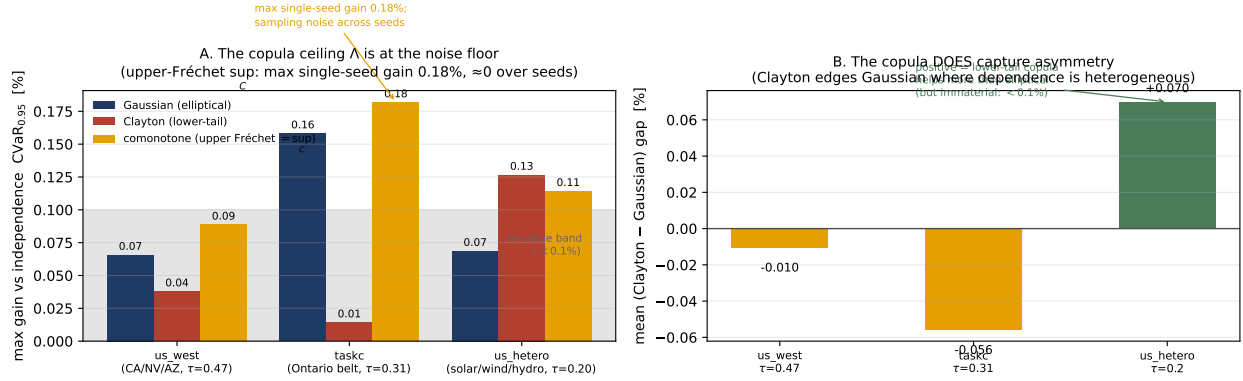
Figure 9: Phase 2 result (single locked scenario seed). A: maximum positive gain versus independence for the Gaussian, Clayton, and comonotone (upper-Fréchet \sup_C ) arms. The largest single-seed comonotone gain is 0.18% (taskc); re-evaluated over scenario seeds it is sampling noise centred on zero (Figure 11). B: the mean Clayton–Gaussian increment by grid; positive where dependence is heterogeneous (us_hetero, +0.07%), confirming the copula does capture the asymmetry, but an order of magnitude too small to matter, as Proposition 1 predicts.
