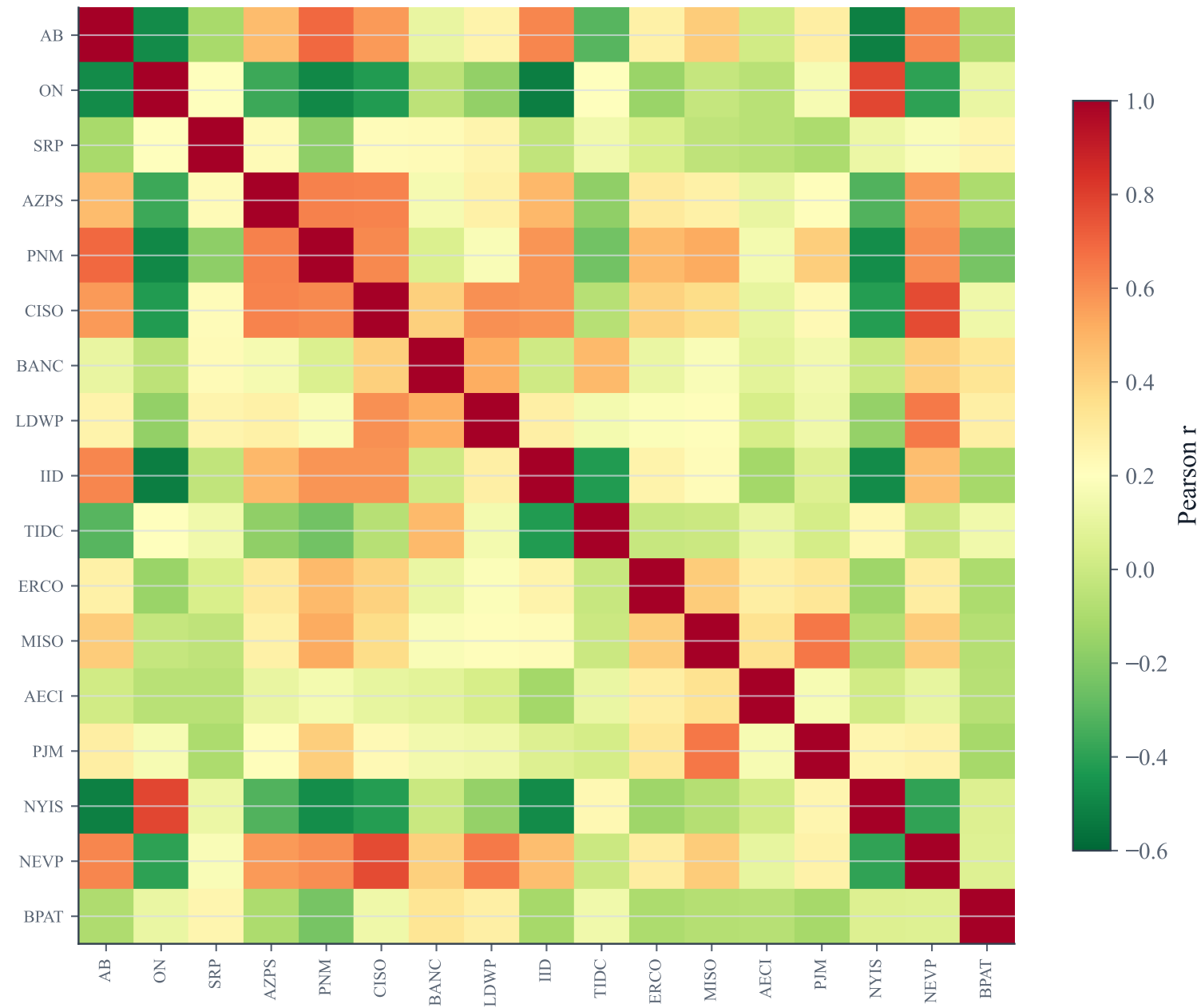
De-seasonalized carbon-intensity correlation, 17 NA zones
