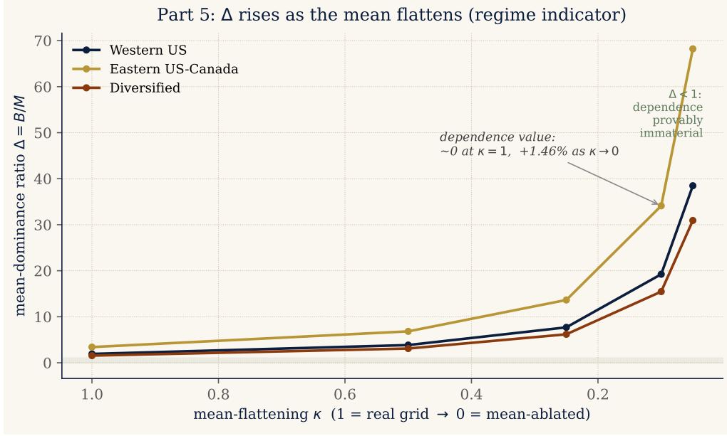
Figure 16: Part 5. The mean-dominance ratio \Delta = B/M along a mean-flattening sweep ( \kappa = 1 real grid \rightarrow \kappa \rightarrow 0 mean-ablated). \Delta rises monotonically as the mean weakens, tracking the empirical dependence value ( \approx 0 on real grids, +1.46\% ablated); the shaded band marks the \Delta < 1 region where dependence is provably immaterial.
