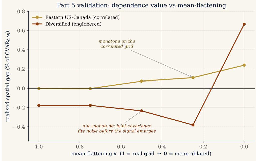
Figure 15: Interior validation of the Part 5 condition. Realised spatial gap (% of \text{CVaR}_{0.95} ) from re-solving the DRO at intermediate mean-flattening \kappa . On the correlated Eastern grid the gap rises monotonically as the mean weakens ( \kappa \rightarrow 0 ), tracking \Delta ; on the engineered Diversified grid it is non-monotone, the joint covariance fitting noise before the true signal emerges, so \Delta orders the regimes only coarsely.
