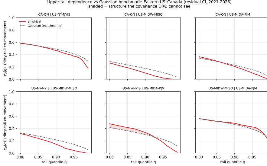
Figure 9: Upper-tail dependence \chi_U(q) for the Ontario–Eastern belt region pairs (solid) against the Gaussian-copula benchmark at the matched correlation (dashed). The empirical curves sit at or below the benchmark as q \rightarrow 1 : in the dirtiest hours the regions decouple, so there is no exploitable upper-tail co-movement for a richer ambiguity set to capture. The complementary radial asymmetry ( \chi_L > \chi_U ) is quantified in Table 6.
