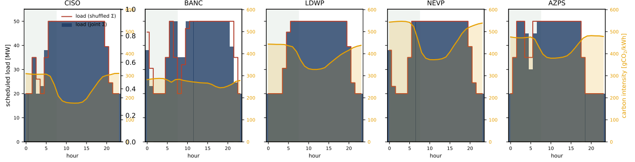
Figure 7: The spatial null, seen directly (Western US, regime R3, \alpha = 0.5 , \varepsilon^* = 1 ). Bars are the optimal load under the joint covariance; the red step is the load under the shuffled (block-diagonal) covariance. The two coincide. The gold curve is each region’s mean carbon intensity; the green band marks the deadline window [0, 7] .
