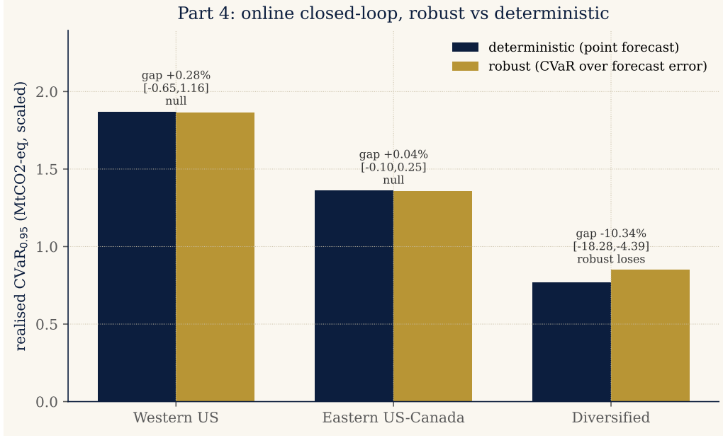
Figure 14: Part 4. Realised closed-loop \text{CVaR}_{0.95} , deterministic vs robust controller, per grid; annotations give the robust gap and its 95% CI. Robustness is null on the correlated grids and counterproductive on the structureless one.
