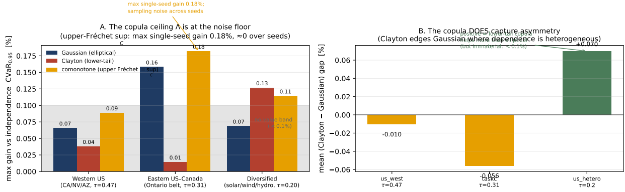
Figure 11: Phase 2 result (single locked scenario seed). A: maximum positive gain versus independence for the Gaussian, Clayton, and comonotone (upper-Fréchet sup C ) arms. The largest single-seed comonotone gain is 0.18% (Eastern US-Canada); re-evaluated over scenario seeds it is sampling noise centred on zero (Figure 17). B: the mean Clayton-Gaussian increment by grid; positive where dependence is heterogeneous (Diversified, +0.07%), confirming the copula does capture the asymmetry, but an order of magnitude too small to matter, as Proposition 1 predicts.
