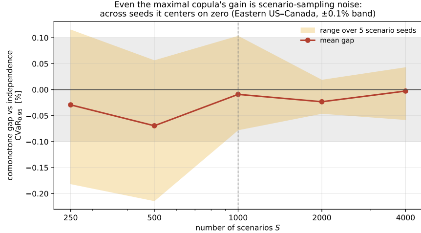
Figure 19: The comonotone gap is scenario-sampling noise. Mean (line) and range over five seeds (band) of the comonotone-vs-independence CVaR_{0.95} gap on Eastern US–Canada, against the scenario count S . The band straddles zero and narrows with S ; the \pm 0.1\% no-value band is shaded.
