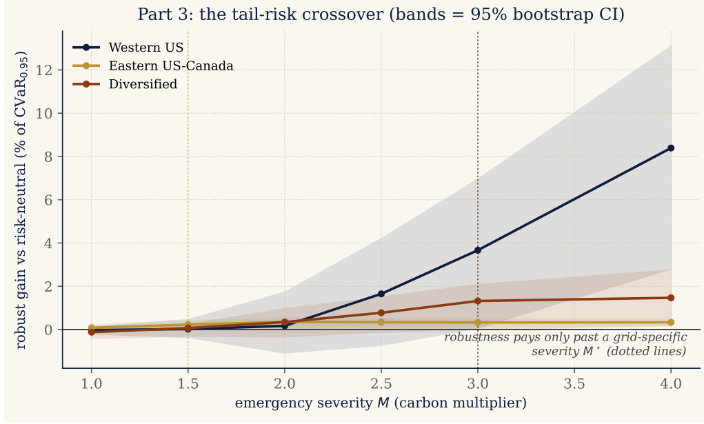
Figure 13: The tail-risk crossover, with uncertainty. Robust-minus-risk-neutral gain (% of \text{CVaR}_{0.95} ) against emergency severity M ; shaded bands are 95% paired-bootstrap intervals, dotted verticals mark each grid's crossover threshold M^* . Robustness is null at M = 1 everywhere and pays only once emergencies are severe enough.
