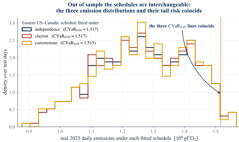
Figure 22: Out of sample the copula schedulers are interchangeable (Eastern US–Canada). Distribution of real 2025 daily emissions under the schedule fitted to independence, Clayton, and comonotone scenarios; the dotted lines mark each \text{CVaR}_{0.95} . All three coincide.
