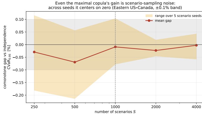
Figure 12: The comonotone gap is scenario-sampling noise. Mean (line) and range over five seeds (band) of the comonotone-vs-independence CVaR_{0.95} gap on Eastern US–Canada, against the scenario count S . The band straddles zero and narrows with S ; the \pm 0.1\% materiality band is shaded.
