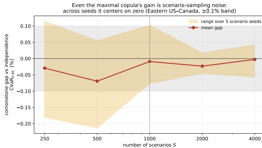
Figure 17: The comonotone gap is scenario-sampling noise. Mean (line) and range over five seeds (band) of the comonotone-vs-independence CVaR_{0.95} gap on Eastern US–Canada, against the scenario count S . The band straddles zero and narrows with S ; the \pm 0.1\% no-value band is shaded.
