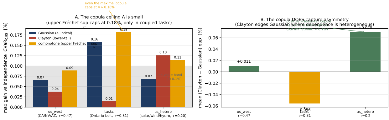
Figure 8: Phase 2 result. A: maximum positive gain versus independence for the Gaussian, Clayton, and comonotone (upper-Fréchet sup C ) arms. The comonotone ceiling \Lambda caps at 0.18%, and only in the coupled belt (taskc); the fitted copulas do not even reach it. B: the mean Clayton–Gaussian increment by grid; positive where dependence is heterogeneous (us_hetero, +0.07%), confirming the copula does capture the asymmetry, but an order of magnitude too small to matter, as Proposition 1 predicts.
