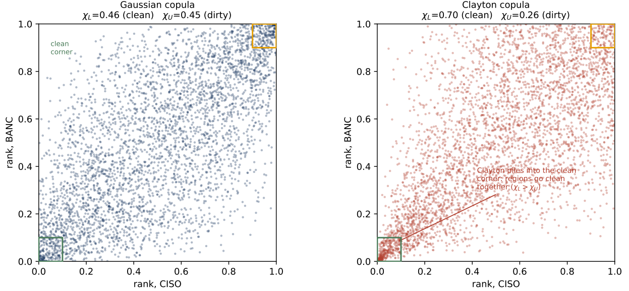
Figure 7: The dependence object a covariance ball cannot represent. Samples from the Gaussian copula (left, symmetric: \chi_L \approx \chi_U ) and the fitted Clayton copula (right) for a representative US-West pair. Clayton concentrates in the lower-left “clean” corner ( \chi_L > \chi_U ), reproducing the Phase 1 radial asymmetry that elliptical models force to zero.
