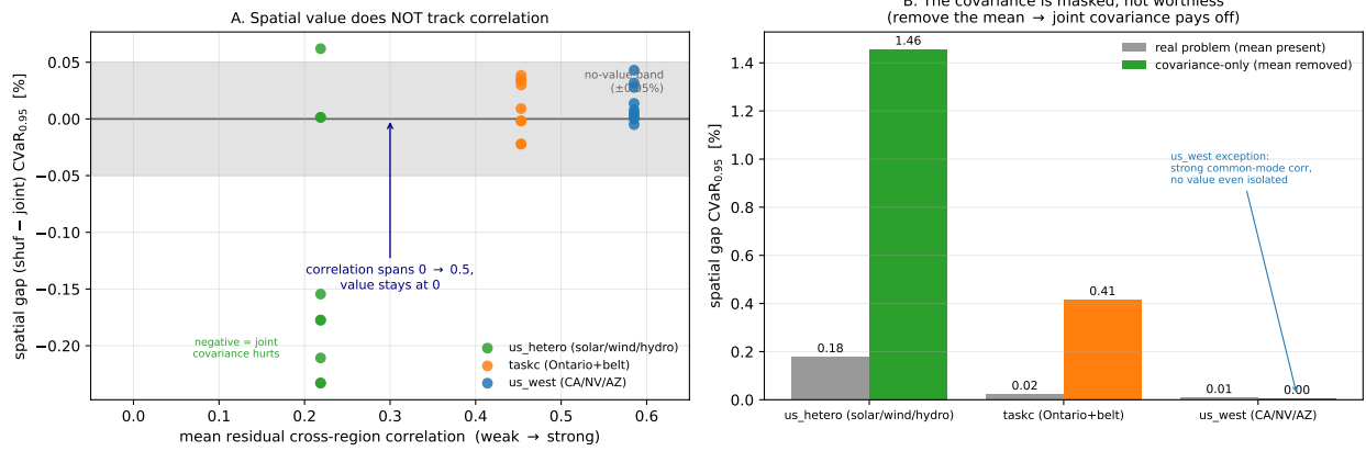
Figure 3: The Phase 1 finding. A: spatial gap vs. mean residual cross-region correlation; value does not track correlation anywhere on the spectrum. B: mean-ablation; in the covariance-only world (constant scheduling mean) the joint covariance pays off by up to +1.46%, proving the spatial signal is real but masked by the mean carbon field, not absent.
