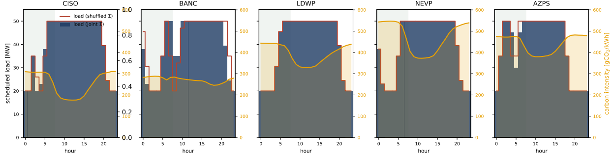
Figure 4: The spatial null, seen directly (us_west, regime R3, \alpha = 0.5 , \varepsilon^* = 1 ). Bars are the optimal load under the joint covariance; the red step is the load under the shuffled (block-diagonal) covariance. The two coincide. The gold curve is each region’s mean carbon intensity; the green band marks the deadline window [0, 7] .
