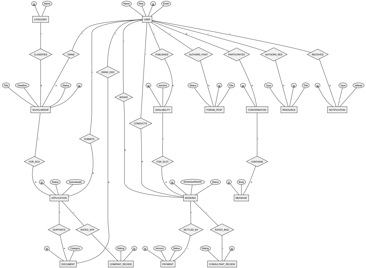
Figure 1: The basic conceptual ERD for ScholarPath in Chen / Elmasri notation — the deliberately plain starting point. USER is a single flat entity whose Role is just an attribute.
