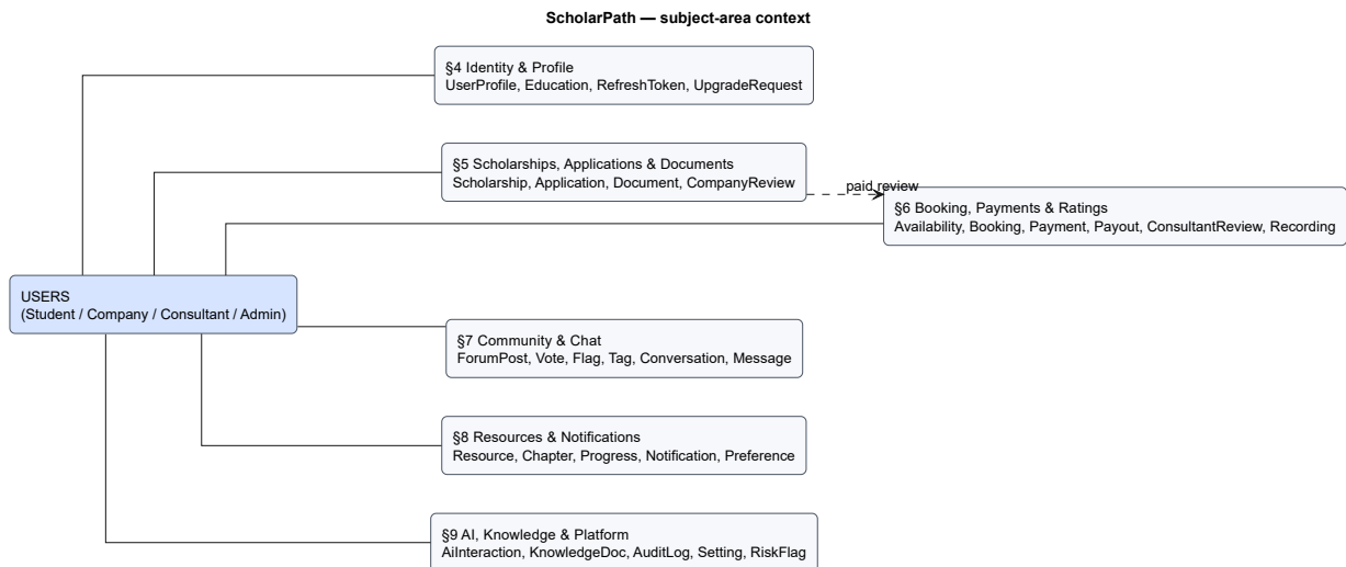
Figure 2: Subject-area context. Everything radiates from USER ; each cluster is detailed in the later parts of this series.
