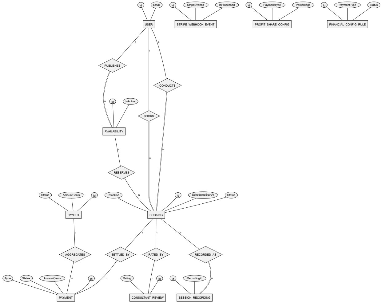
Figure 5: Booking, Payments & Ratings cluster (Chen / Elmasri notation).
