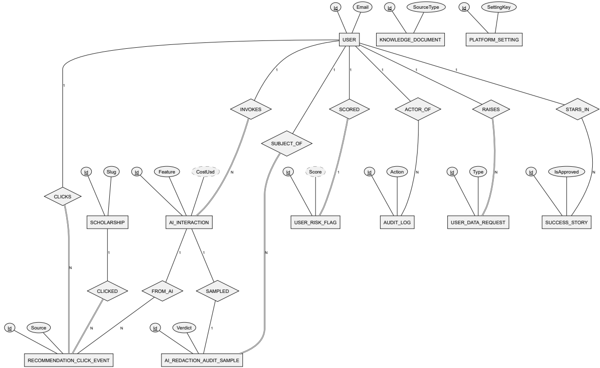
Figure 8: AI, Knowledge Base & Platform cluster (Chen / Elmasri notation).
