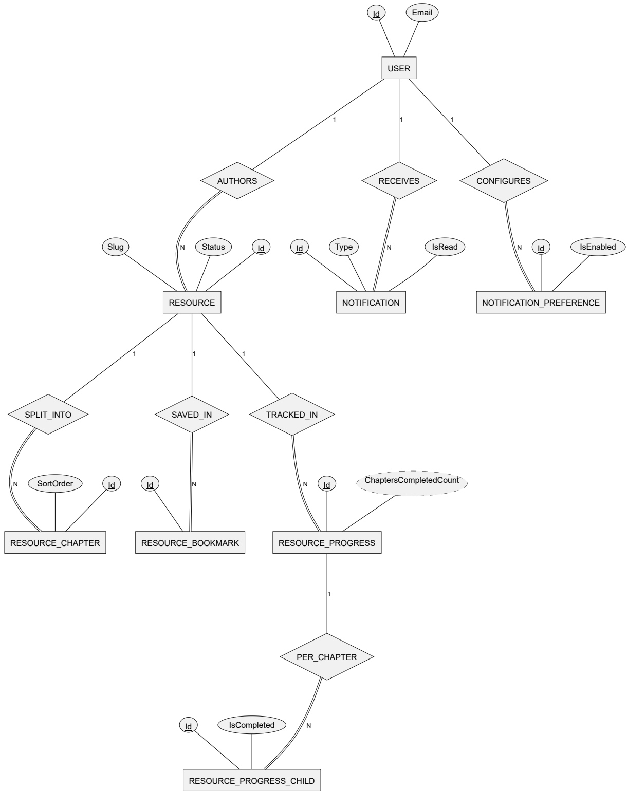
Figure 7: Resources Hub & Notifications cluster (Chen / Elmasri notation).
