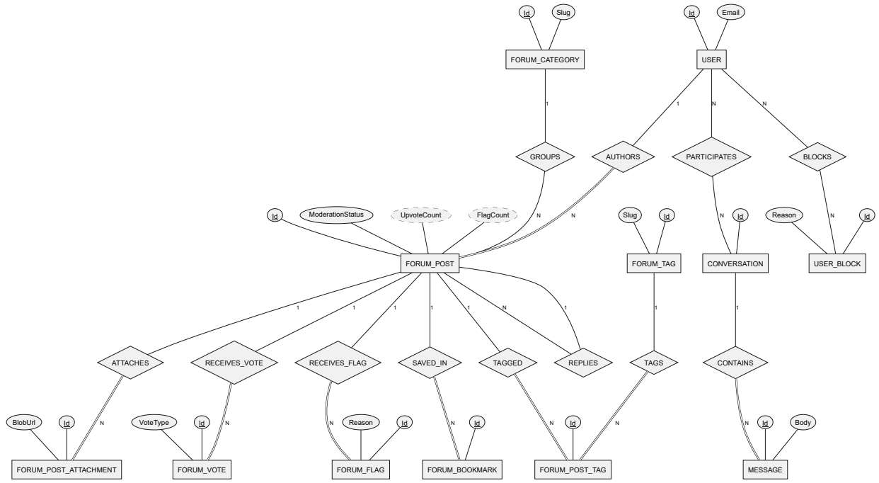
Figure 6: Community & Chat cluster (Chen / Elmasri notation).
