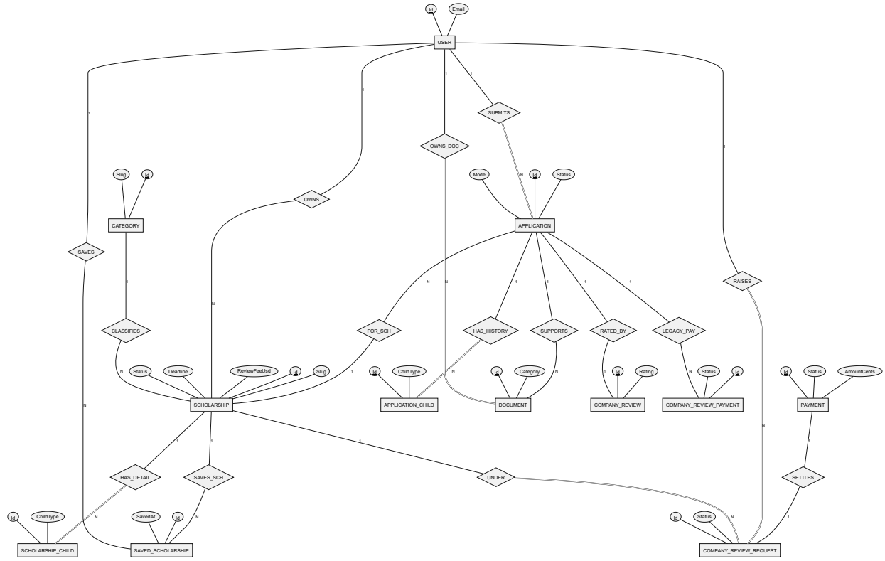
Figure 4: Scholarships, Applications & Documents cluster (Chen / Elmasri notation).
