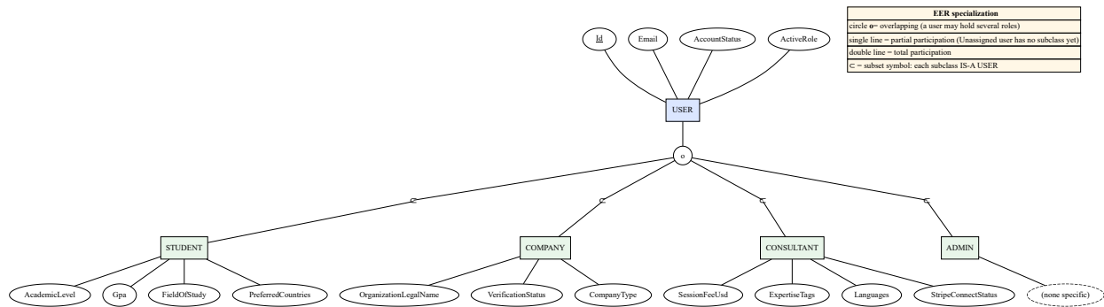
Figure 1: The USER super-type specialized into Student, Company, Consultant and Admin in authentic Elmasri & Navathe EER notation. The specialization circle carries o (overlapping); the single line from USER to the circle marks partial participation; each subset symbol ( \subset ) reads “subclass IS-A USER”.
