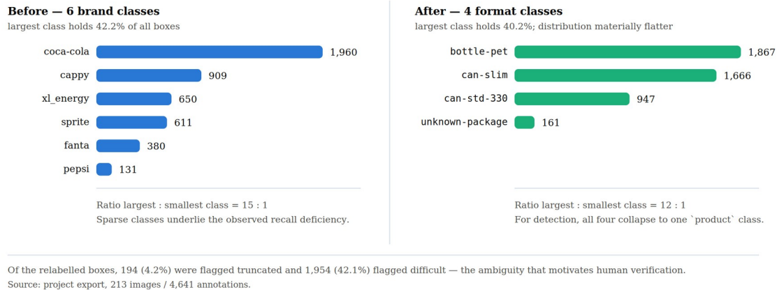
Figure 2. Annotation distribution before and after geometric relabelling. The same 4,641 boxes are partitioned by manufacturer brand (left) and by physical packaging format (right).
