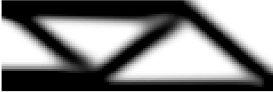
Figure 29: Nearest-neighbor upsampled coarse-resolution OC design optimized on a 120 \times 40 analysis-density mesh with a physically equivalent filter radius r_{\min} = 4.8 coarse elements.
