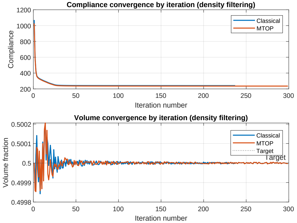
Figure 13: Classical and MTOP OC convergence histories versus iteration number, for density filtering. The compliance is well-stabilized after about fifty iterations, but the maximum design change cannot reach the \varepsilon = 0.01 tolerance within the iteration budget for either formulation.
