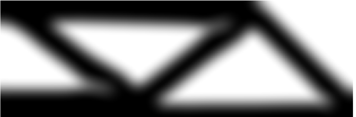
Figure 10: Optimized classical OC design with density filtering on a 600 \times 200 mesh, V^* = 0.5 , p = 3 and r_{\min} = 24 density cells. The grey halo around each member width corresponds to the filter radius and reflects the minimum length scale enforced by the density filter.
