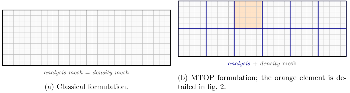
Figure 1: Classical and MTOP discretizations at aspect ratio 3:1.
