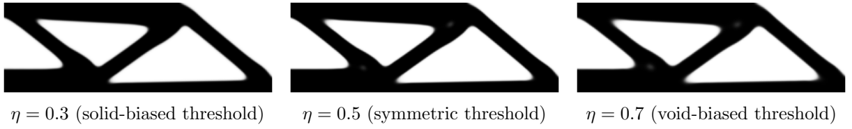
Figure 17: Optimized MTOP MMA designs with Heaviside projection for the three threshold values \eta used in step 4.
