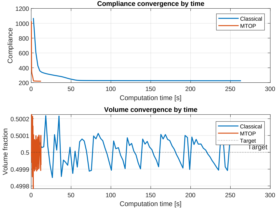
Figure 9: Classical and MTOPT OC convergence histories versus wall-clock time. The MTOPT curve is compressed against the left axis because each iteration solves a much smaller equilibrium problem.
