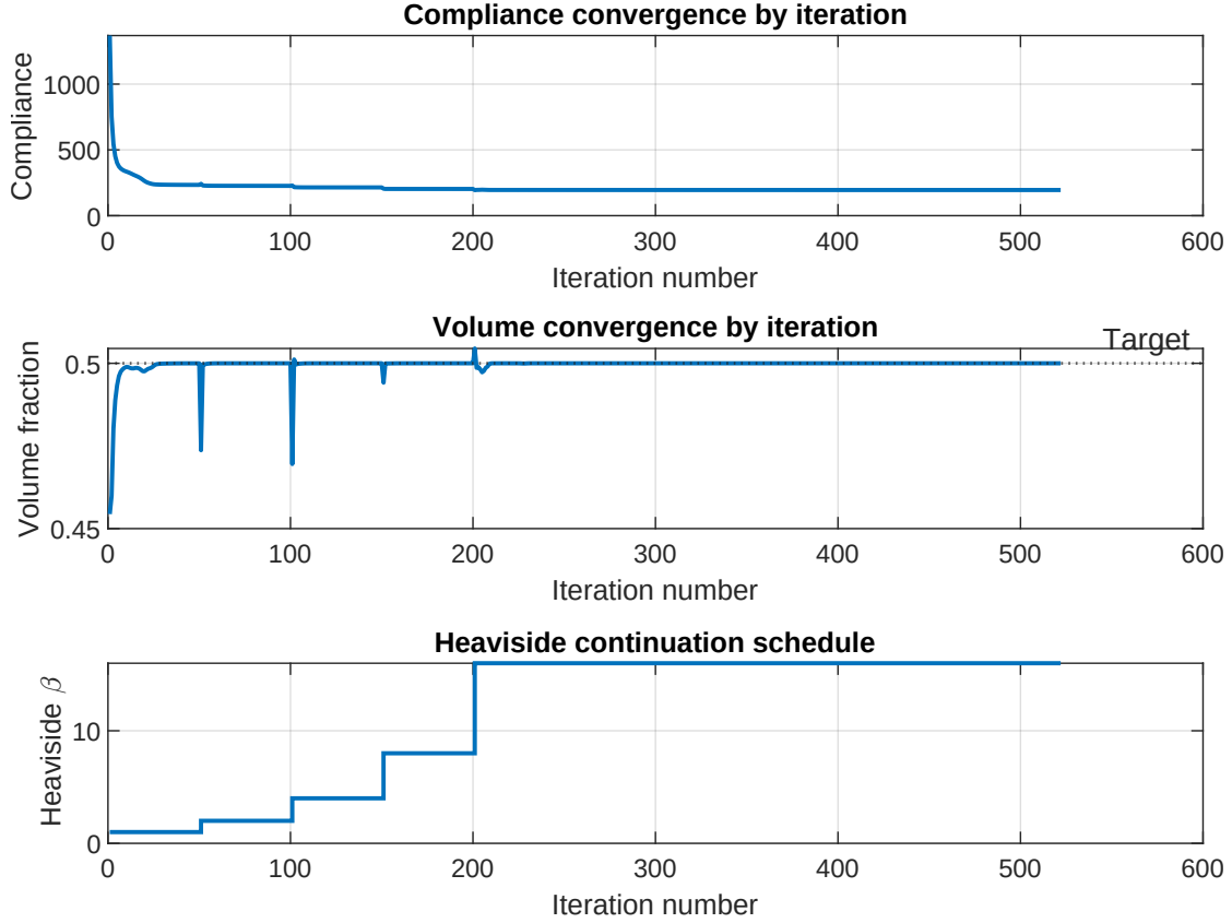
Figure 20: Convergence history for the void-biased Heaviside run ( \eta = 0.7 ): compliance, volume fraction and the continuation parameter \beta versus iteration number.
