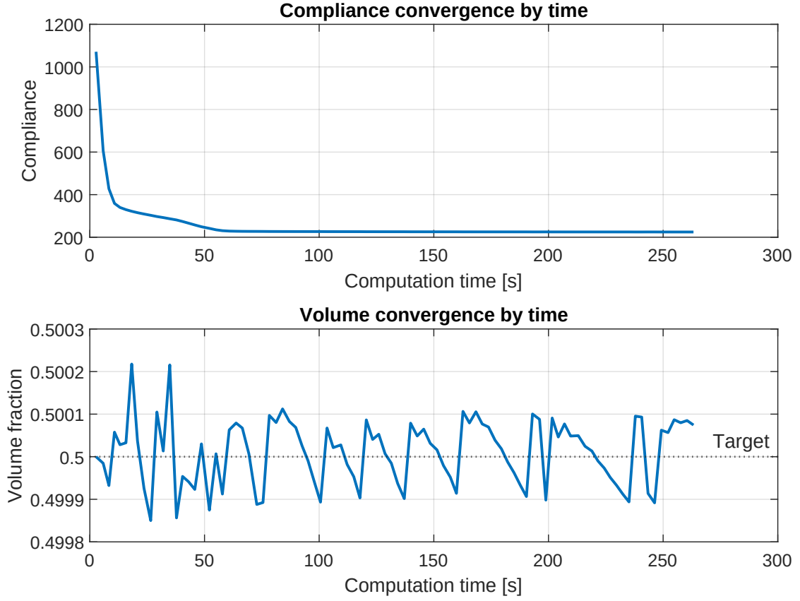
Figure 5: Classical OC convergence history versus elapsed wall-clock time: compliance (top) and volume fraction (bottom). The same data are used in fig. 9 for the runtime comparison with MTOP.
