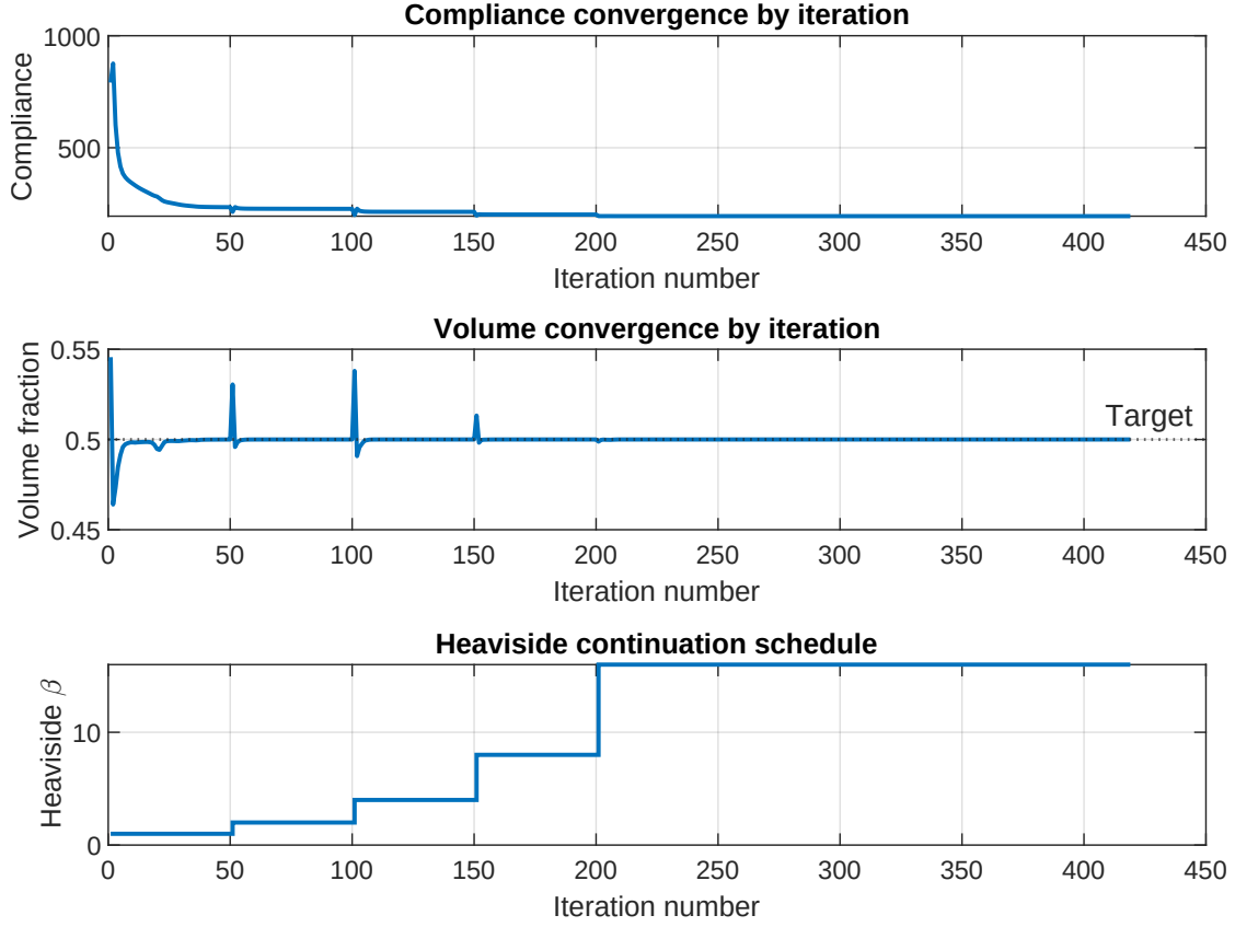
Figure 19: Convergence history for the solid-biased Heaviside run ( \eta = 0.3 ): compliance, volume fraction and the continuation parameter \beta versus iteration number.
