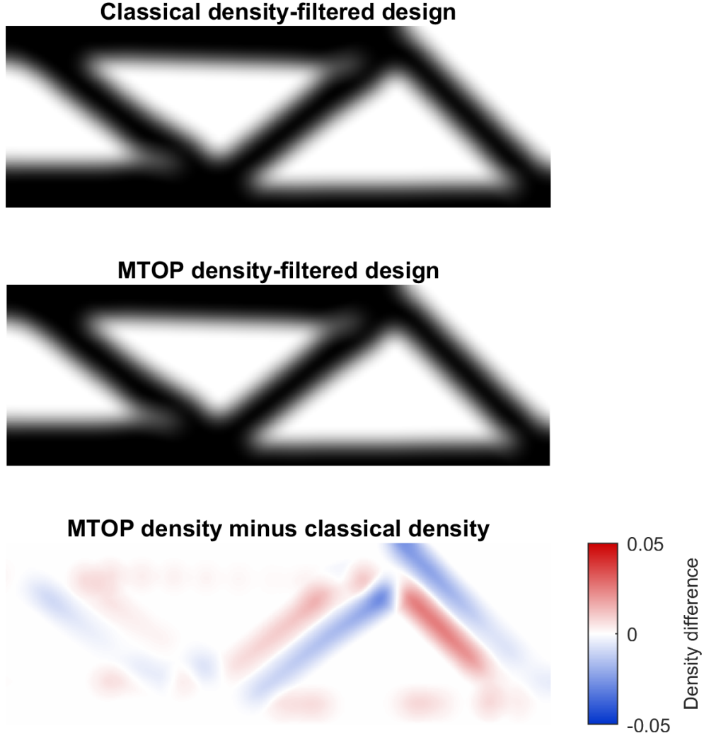
Figure 12: Comparison of the classical and MTOP OC designs with density filtering (top, middle) and signed density difference \rho_{\text{mtop}} - \rho_{\text{cl}} (bottom). The maximum absolute density difference is 0.0065, the RMS difference is 0.0010 and the mean absolute density difference is 0.0005. The differences are markedly smaller than for sensitivity filtering (fig. 7) because the density filter pre-smooths the design variables before the SIMP analysis, so the choice of integration scheme inside the analysis element has less effect on the resulting layout.
