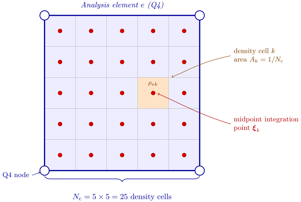
Figure 2: Anatomy of one MTOP analysis element.
