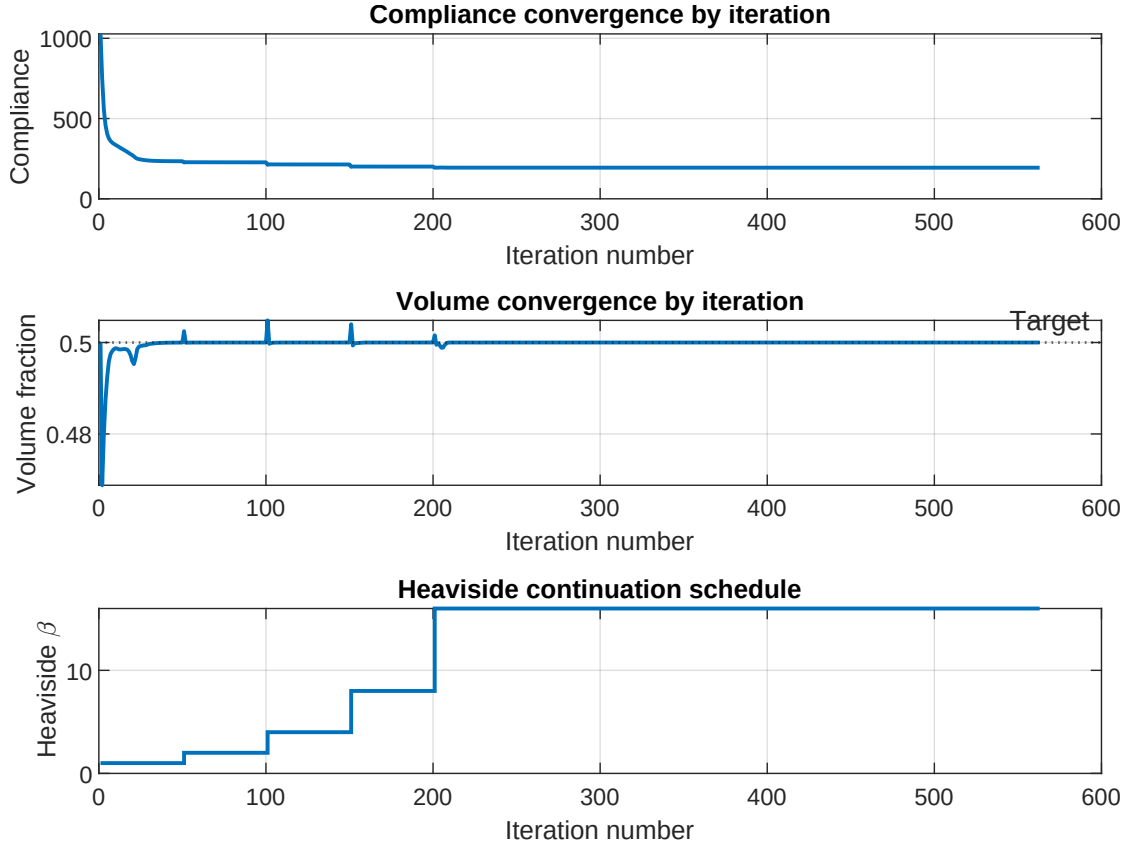
Figure 18: Convergence history for the symmetric Heaviside run ( \eta = 0.5 ): compliance, volume fraction and the continuation parameter \beta versus iteration number. Each \beta doubling corresponds to a small jump in the compliance because the projection becomes sharper. The final design is reached at \beta = \beta_{\max} = 16 .
