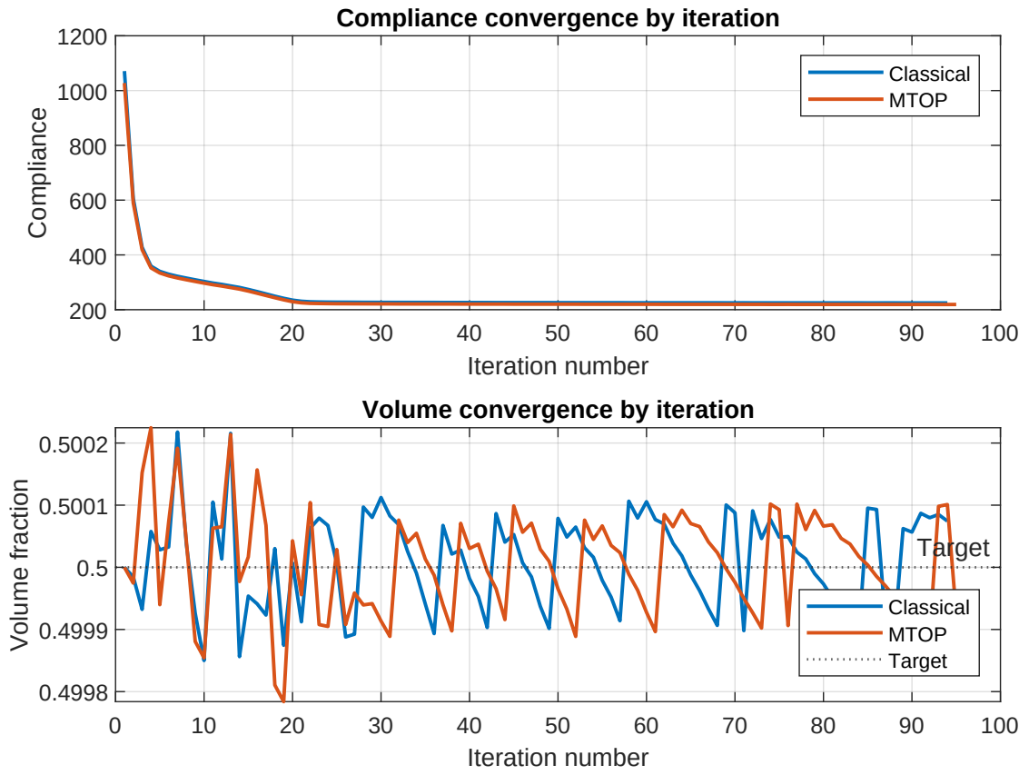
Figure 8: Classical and MTOP OC convergence histories versus iteration number. The two histories are nearly indistinguishable.
