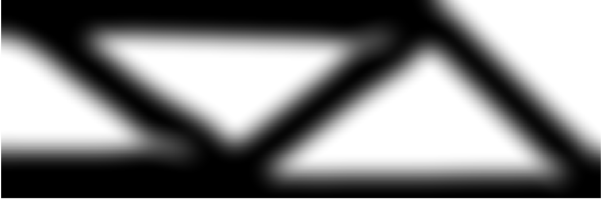
Figure 11: Optimized MTOP OC design with density filtering, on a 120 \times 40 analysis mesh and 5 \times 5 density cells per analysis element.
