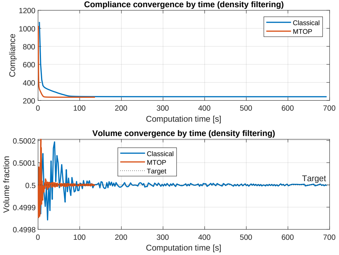
Figure 14: Classical and MTOP OC convergence histories versus wall-clock time, for density filtering. Both runs are stopped by the compliance-stability criterion of Section 4.5, at 237 and 299 iterations respectively; the wall-clock speedup of MTOP over the classical run is 5.07.
