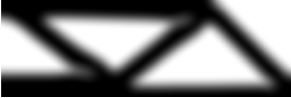
Figure 8: Optimized classical OC design with density filtering on a 600 \times 200 mesh, V^* = 0.5 , p = 3 and r_{min} = 24 density cells. The grey halo around each member width corresponds to the filter radius and reflects the minimum length scale enforced by the density filter.
