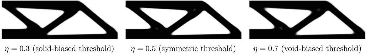
Figure 15: Optimized MTOP MMA designs with Heaviside projection for the three threshold values \eta used in step 4.
