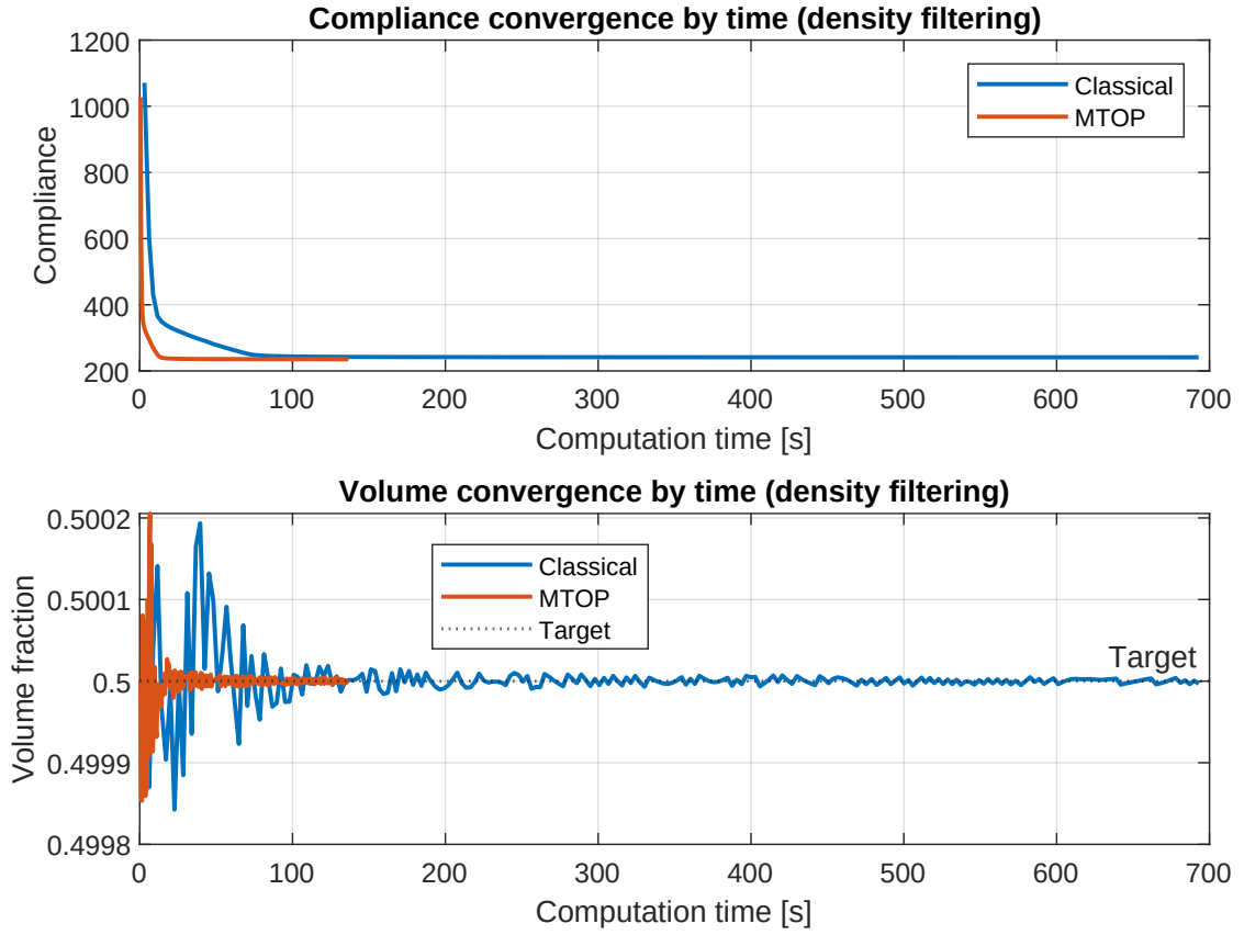
Figure 12: Classical and MTOP OC convergence histories versus wall-clock time, for density filtering. Both runs are stopped by the compliance-stability criterion of Section 4.5, at 237 and 299 iterations respectively; the wall-clock speedup of MTOP over the classical run is 5.07.
