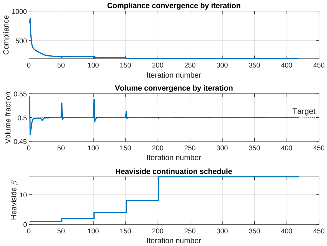
Figure 17: Convergence history for the solid-biased Heaviside run ( \eta = 0.3 ): compliance, volume fraction and the continuation parameter \beta versus iteration number.
