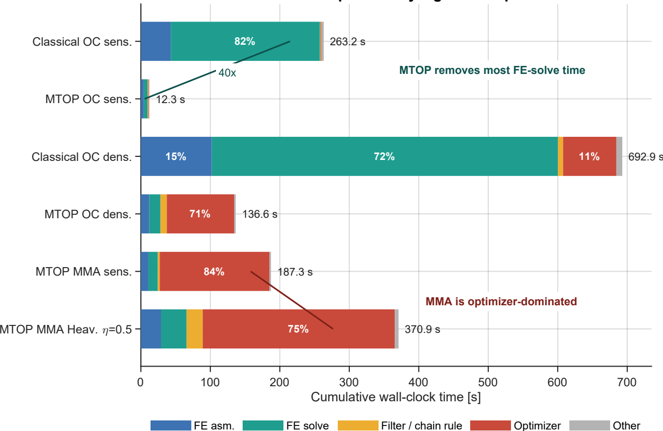
Runtime composition by algorithmic phase
