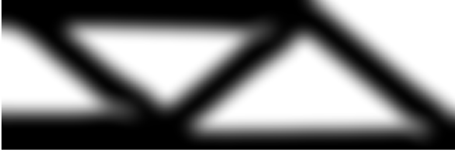
Figure 19: Optimized MTOP MMA design with density filtering.
