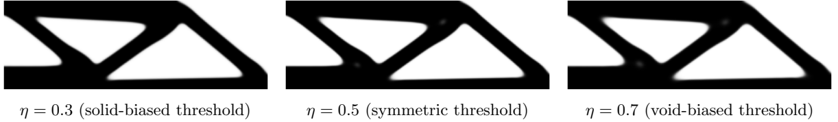
Figure 20: Optimized MTOP MMA designs with Heaviside projection for the three threshold values \eta used in step 4.
