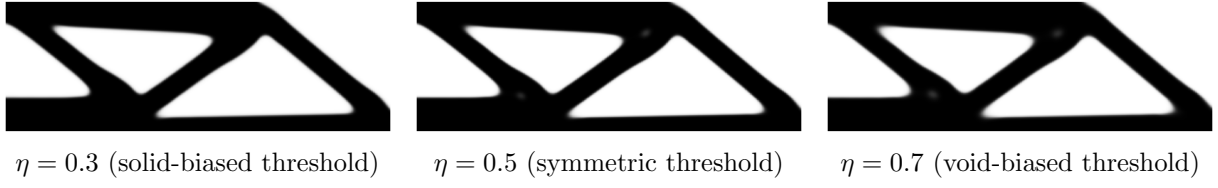
Figure 20: Optimized MTOP MMA designs with Heaviside projection for the three threshold values \eta used in step 4.
