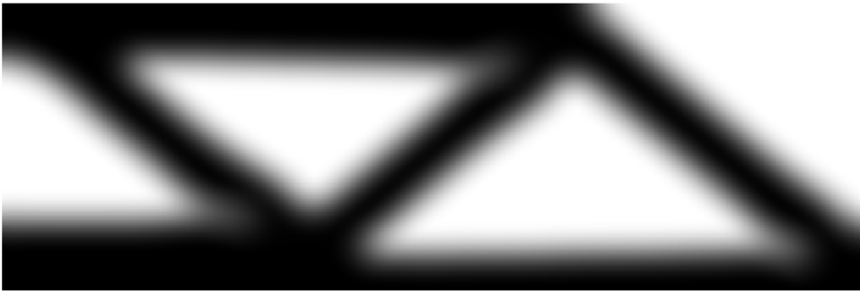
Figure 19: Optimized MTOP MMA design with density filtering.
