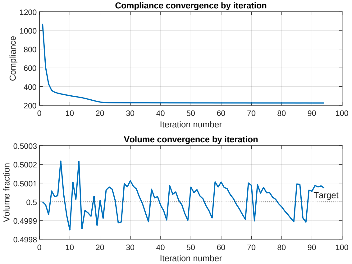
Figure 7: Classical OC convergence history versus iteration number: compliance (top) and volume fraction (bottom).
