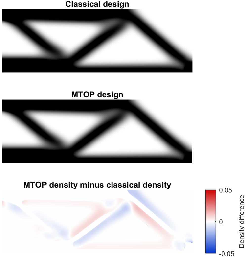
Figure 10: Comparison of the classical and MTOP OC designs (top, middle) and signed density difference \rho_{\text{mtop}} - \rho_{\text{cl}} (bottom). The differences are concentrated on the boundaries of the structural members, where the per-cell midpoint integration of the multiresolution stiffness matrix differs most from the analytical Q4 integration of the classical formulation. The maximum absolute density difference is 0.0222, the RMS difference is 0.0027 and the mean absolute density difference is 0.0013.
