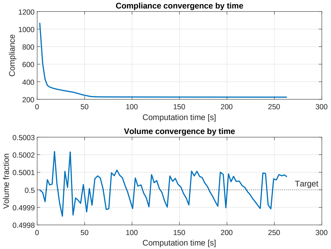
Figure 8: Classical OC convergence history versus elapsed wall-clock time: compliance (top) and volume fraction (bottom). The same data are used in fig. 12 for the runtime comparison with MTOP.
