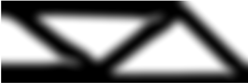
Figure 14: Optimized MTOP OC design with density filtering, on a 120 \times 40 analysis mesh and 5 \times 5 density cells per analysis element.
