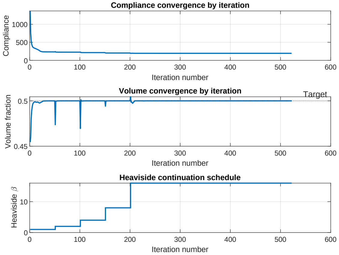
Figure 23: Convergence history for the void-biased Heaviside run ( \eta = 0.7 ): compliance, volume fraction and the continuation parameter \beta versus iteration number.
