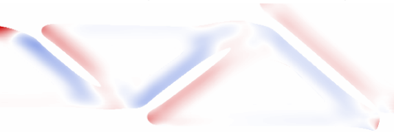
MTOP density minus classical density
