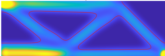
MTOP after density-filter chain rule
