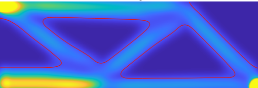
Classical after density-filter chain rule
