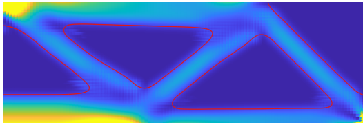
MTOP raw sensitivity
