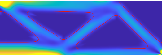
Classical raw sensitivity
