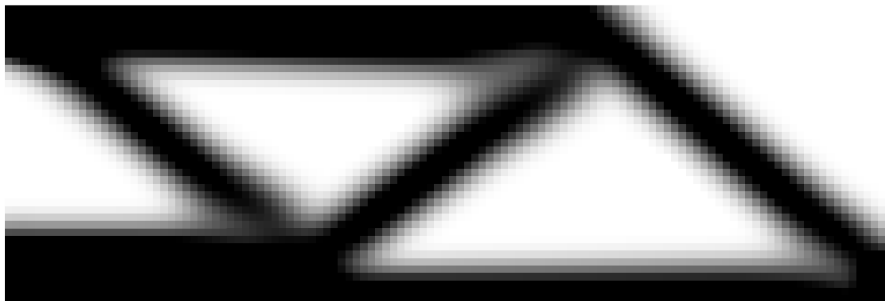
Figure 29: Upsampled coarse-coarse OC design optimized on a 120 \times 40 analysis-density mesh with a physically equivalent filter radius r_{\min} = 4.8 coarse elements.
