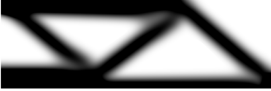
Figure 8: Optimized classical OC design with sensitivity filtering on a 600 \times 200 mesh, V^* = 0.5 , p = 3 and r_{\min} = 24 density cells. Black represents solid material, white represents void.
