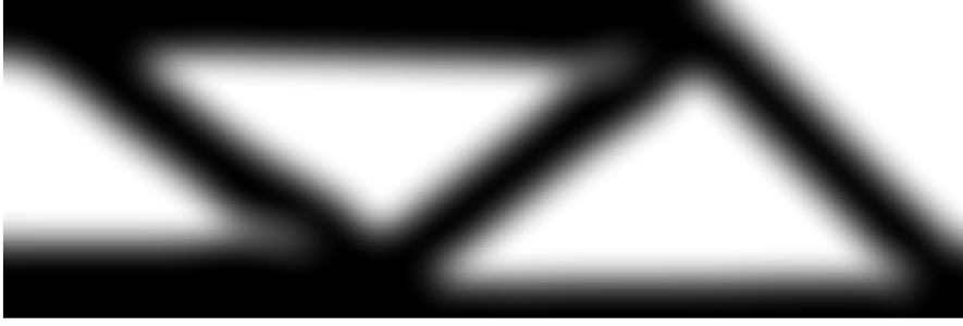
Figure 15: Optimized classical OC design with density filtering on a 600 \times 200 mesh, V^* = 0.5 , p = 3 and r_{\min} = 24 density cells. The grey halo around each member width corresponds to the filter radius and reflects the minimum length scale enforced by the density filter.
