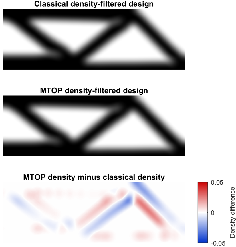
Figure 17: Comparison of the classical and MTOP OC designs with density filtering (top, middle) and signed density difference \rho_{\text{mtop}} - \rho_{\text{cl}} (bottom). The maximum absolute density difference is 0.0065, the RMS difference is 0.0010 and the mean absolute density difference is 0.0005. The differences are markedly smaller than for sensitivity filtering (fig. 12) because the density filter pre-smooths the design variables before the SIMP analysis, so the choice of integration scheme inside the analysis element has less effect on the resulting layout.
