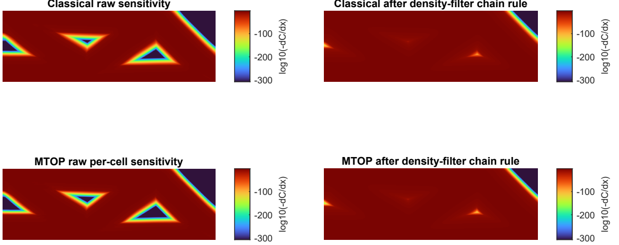
Figure 20: Compliance sensitivity fields at the final density-filtered OC designs. The raw sensitivities -\partial C/\partial \rho are concentrated along the load-carrying members, while the design-variable sensitivities after the density-filter chain rule are smooth over the imposed length scale. The same sensitivity structure is obtained by the classical and MTOP analyses, supporting the use of the compliance-plateau criterion once the residual design-variable change is only a high-frequency boundary oscillation.
