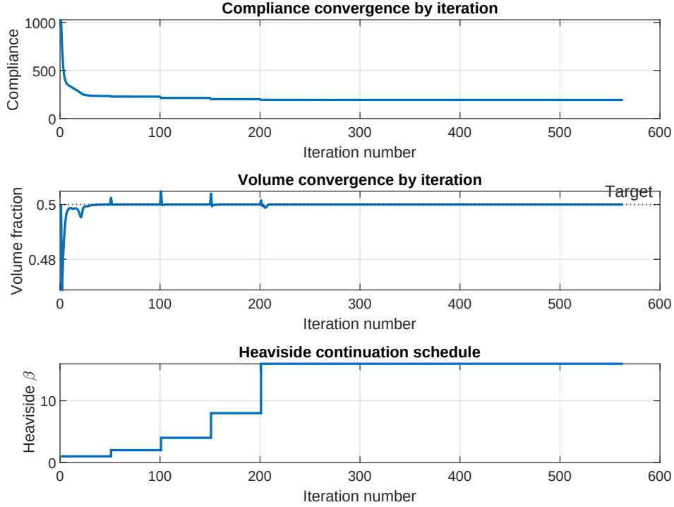
Figure 24: Convergence history for the symmetric Heaviside run ( \eta = 0.5 ): compliance, volume fraction and the continuation parameter \beta versus iteration number. Each \beta doubling corresponds to a small jump in the compliance because the projection becomes sharper. The final design is reached at \beta = \beta_{\max} = 16 .
