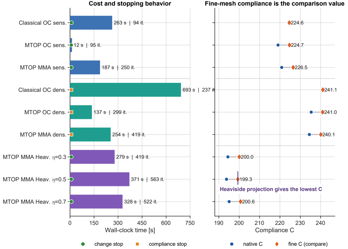
Figure 27: Runtime and compliance summary for the nine runs, sorted by filtering or projection family. The left panel shows cost, iterations and stopping criterion; the right panel uses fine-mesh compliance as the comparison value and shows native compliance only as an auxiliary MTOP diagnostic.
