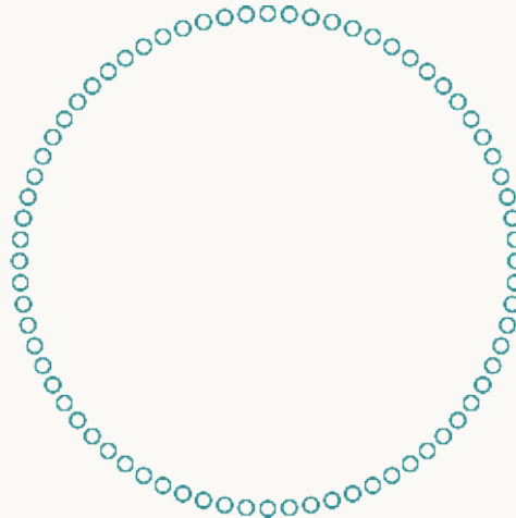
72-direction separated IFS m = 72, r = 0.03 \dim H = 1.219619
