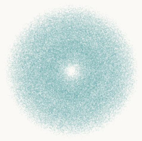
Overlapping 72-direction IFS m = 72, r = 0.5 \dim H not established here
