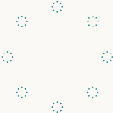
Separated endpoint dust m = 8, r = 0.1 \dim H = 0.903090
