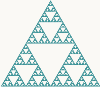
Sierpinski triangle m = 3, r = 0.5 \dim H = 1.584963
