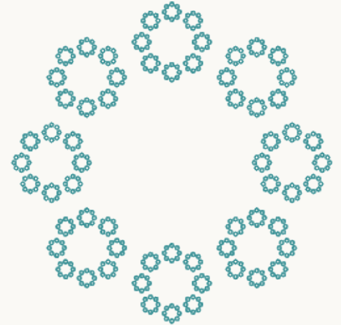
Separated octagonal IFS m = 8, r = 0.25 \dim H = 1.5
