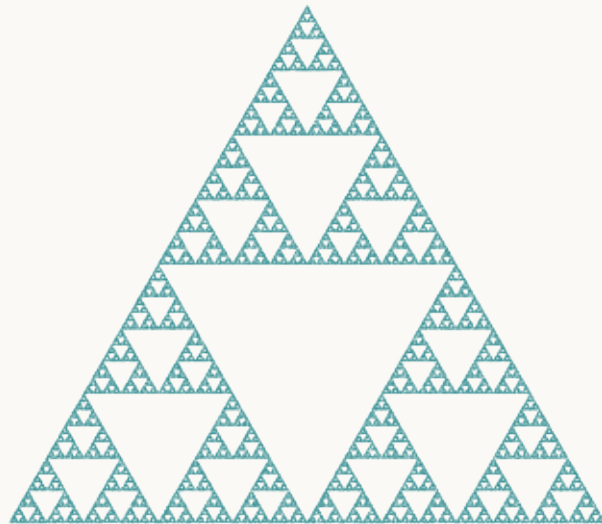
Endpoint-attractor sample K Sierpinski triangle; 100,000 samples
