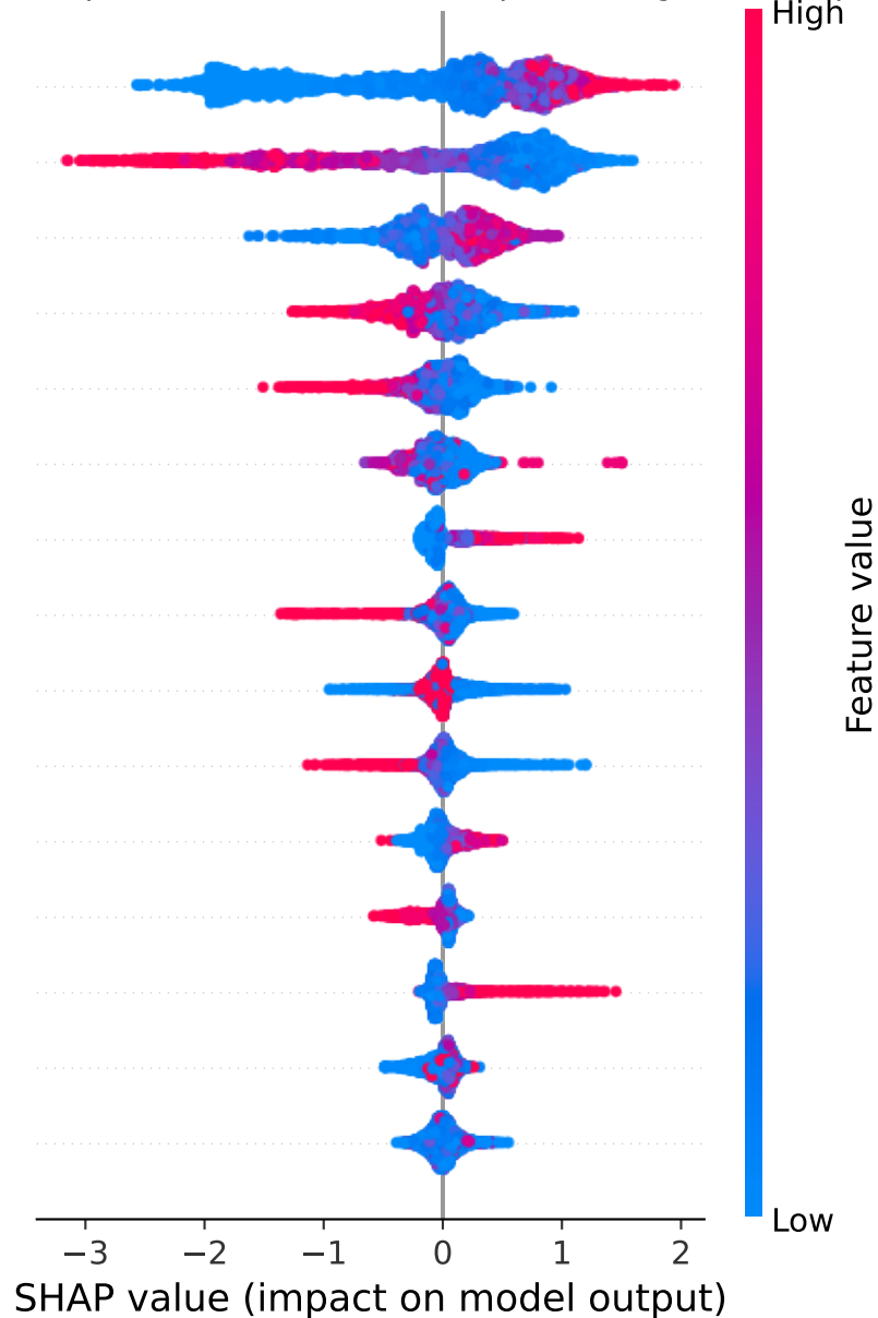
SHAP feature importance - variant: consequence (LightGBM, top 15)
