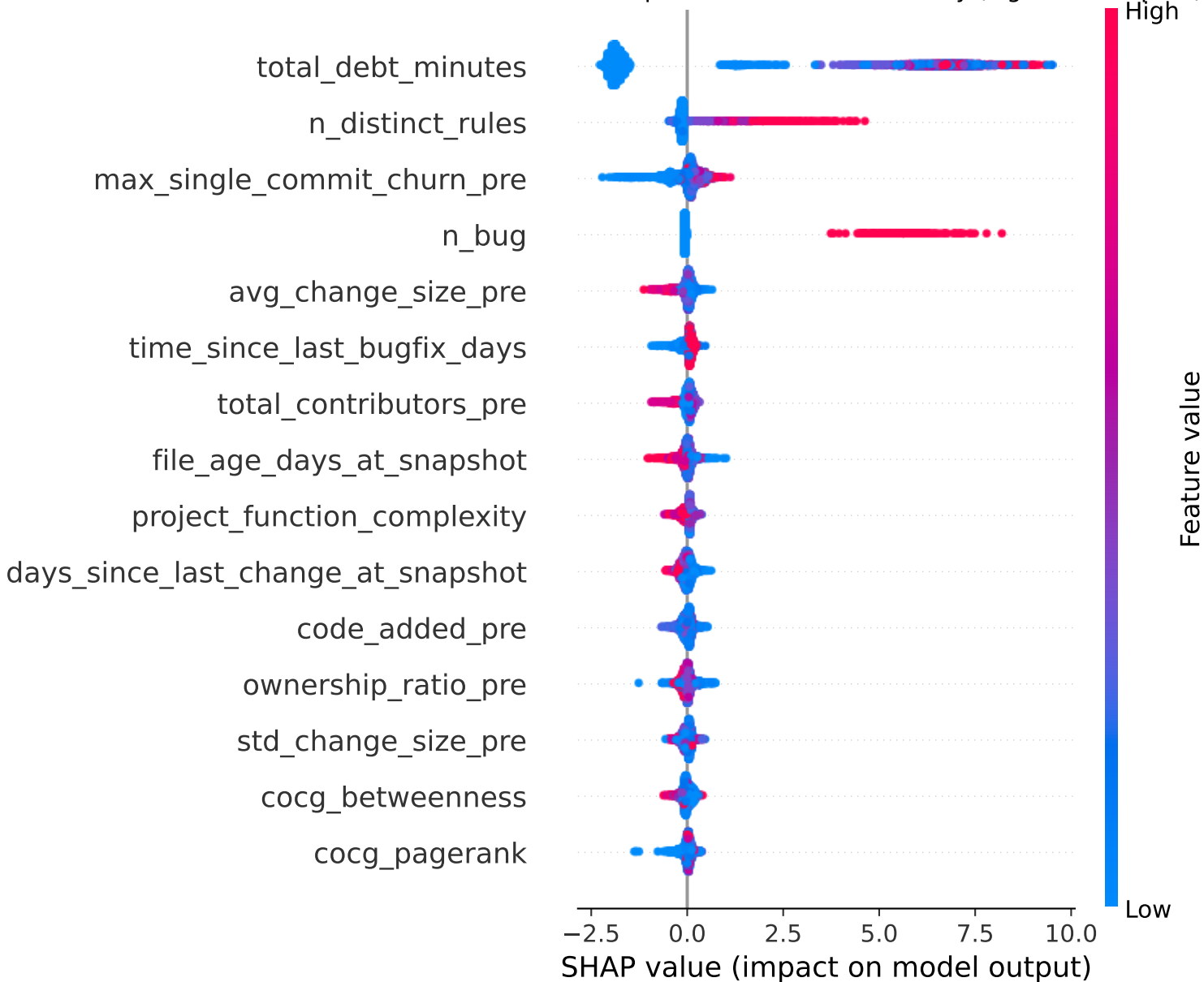
SHAP feature importance - variant: severity (LightGBM, top 15)
