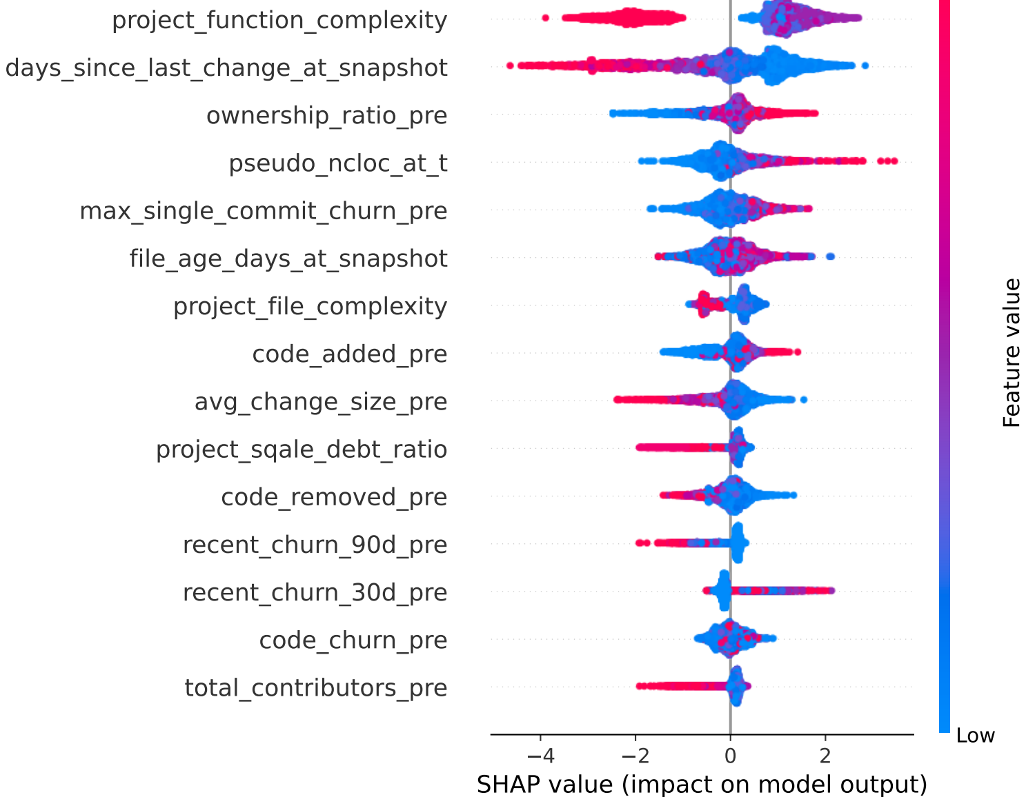
SHAP feature importance - variant: szz (LightGBM, top 15)
