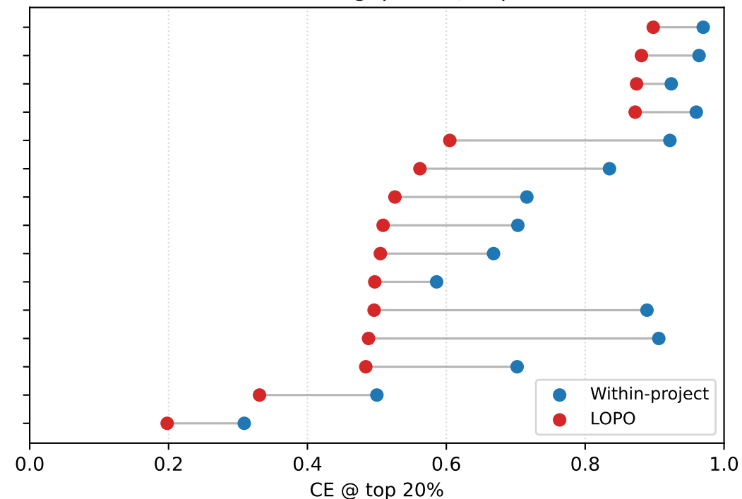
Generalization gap: CE @ top 20%
