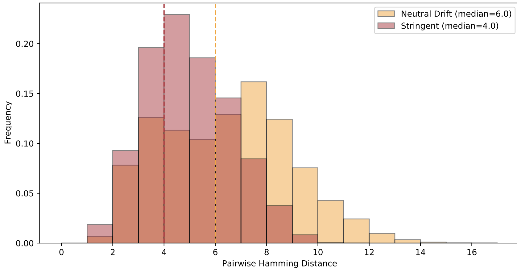
Pairwise AA Hamming Distance Distributions
