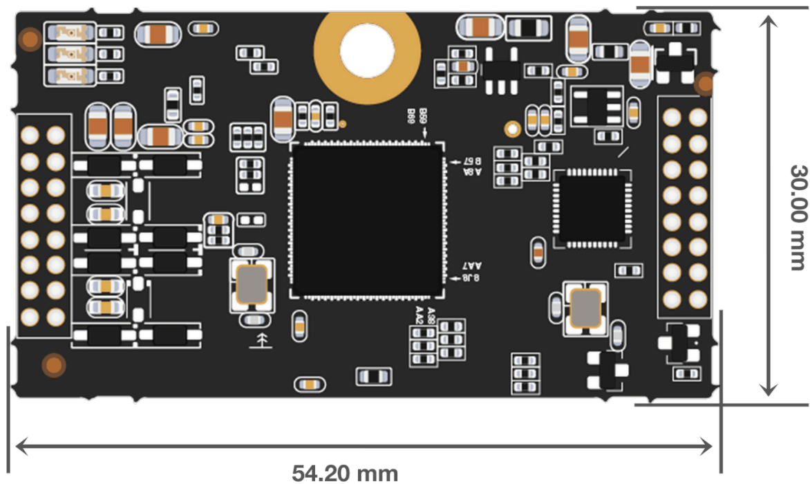
Figure 5: Module dimensions
